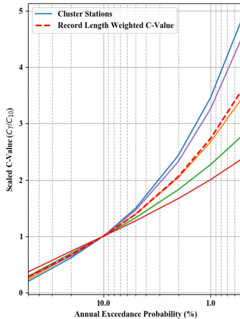
Dimensionless Peak Flow and Scaled C-value - Cluster 30
