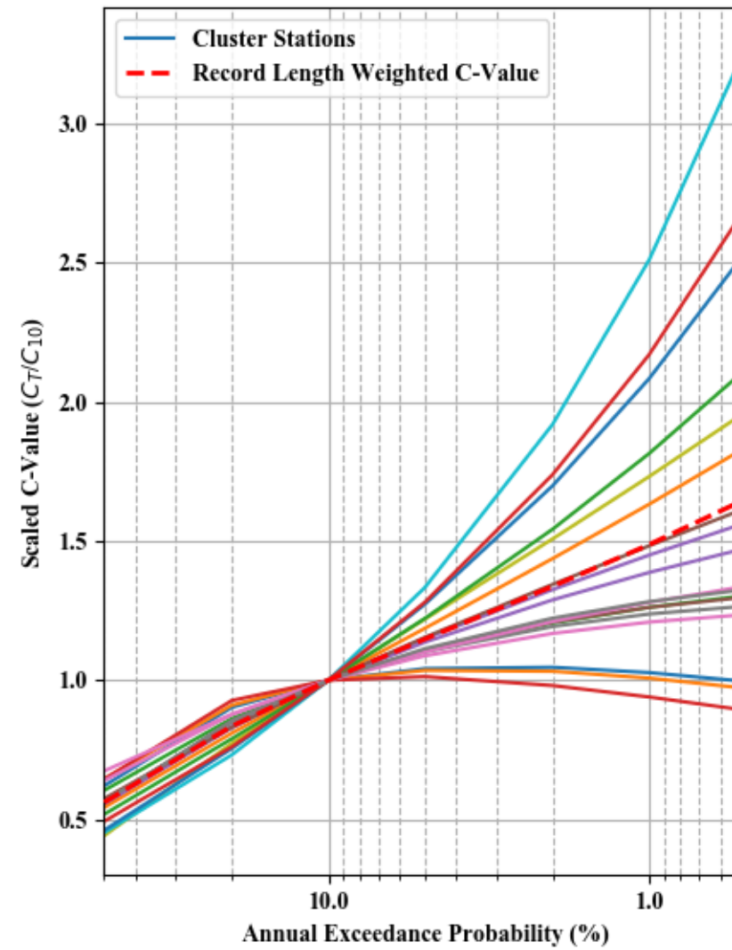
Dimensionless Peak Flow and Scaled C-value - Cluster 35
