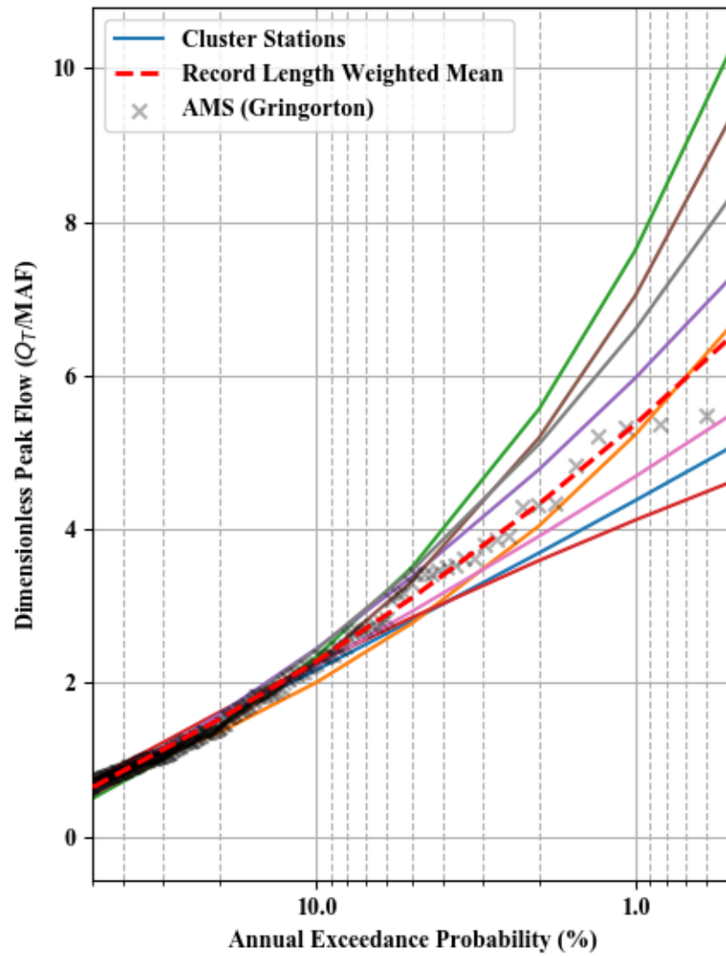
Dimensionless Peak Flow and Scaled C-value - Cluster 10
