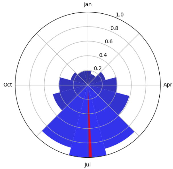
Figure 4.3 Normalised rainfall seasonality for station 0004816AW indicating the monthly (blue) and average (red) rainfall seasonality
