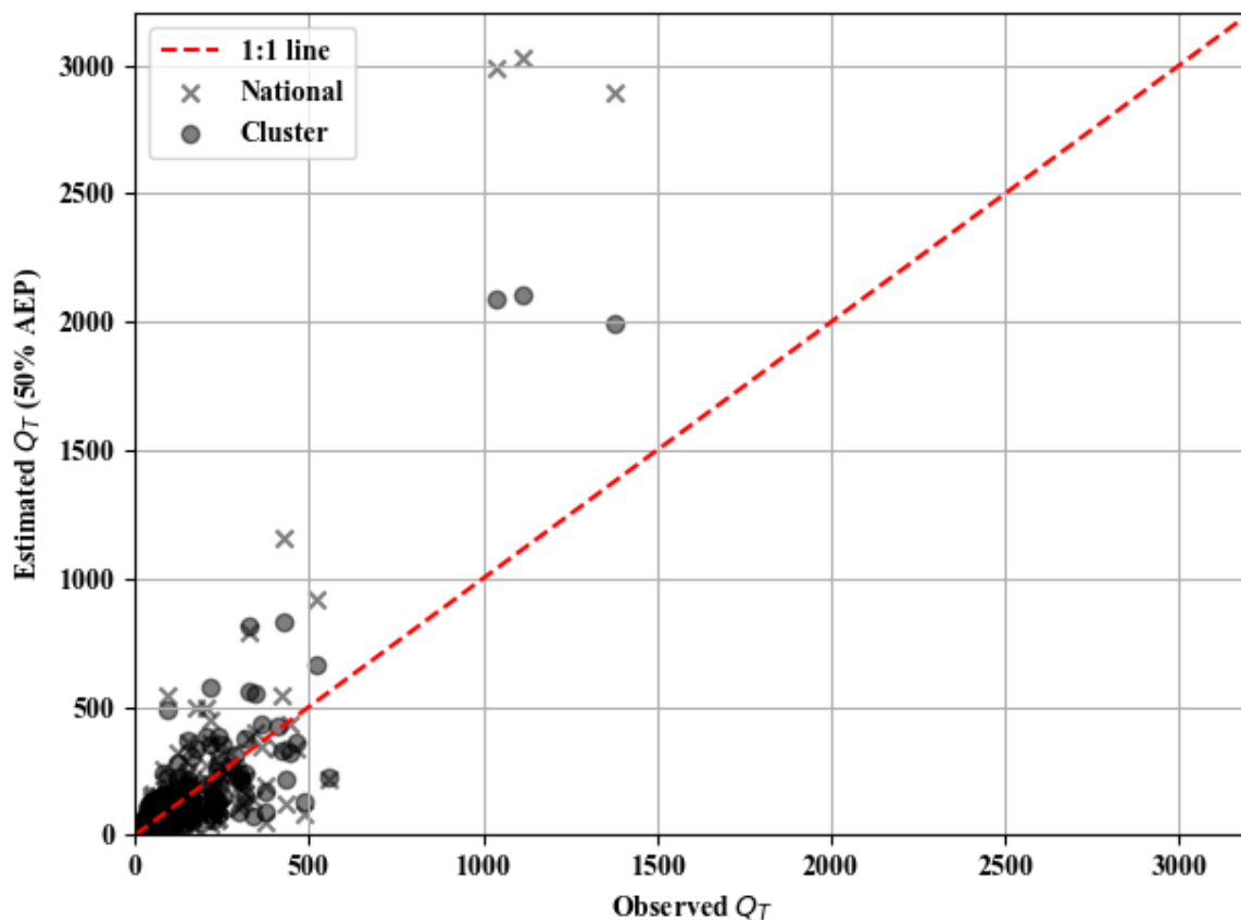
Figure 8.10 Estimated vs observed Q_T using the C_{10} approach for the 50% AEP
