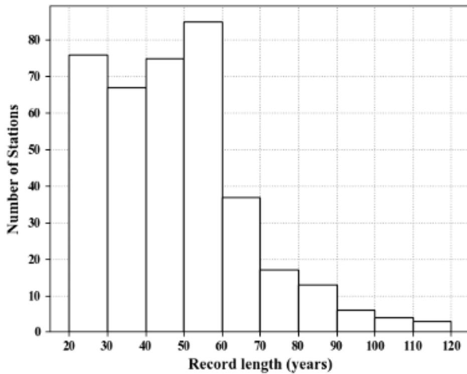
Figure 5.3 Histogram depicting the distribution of the station record lengths for the selected 383 gauging and synthetic dam stations
