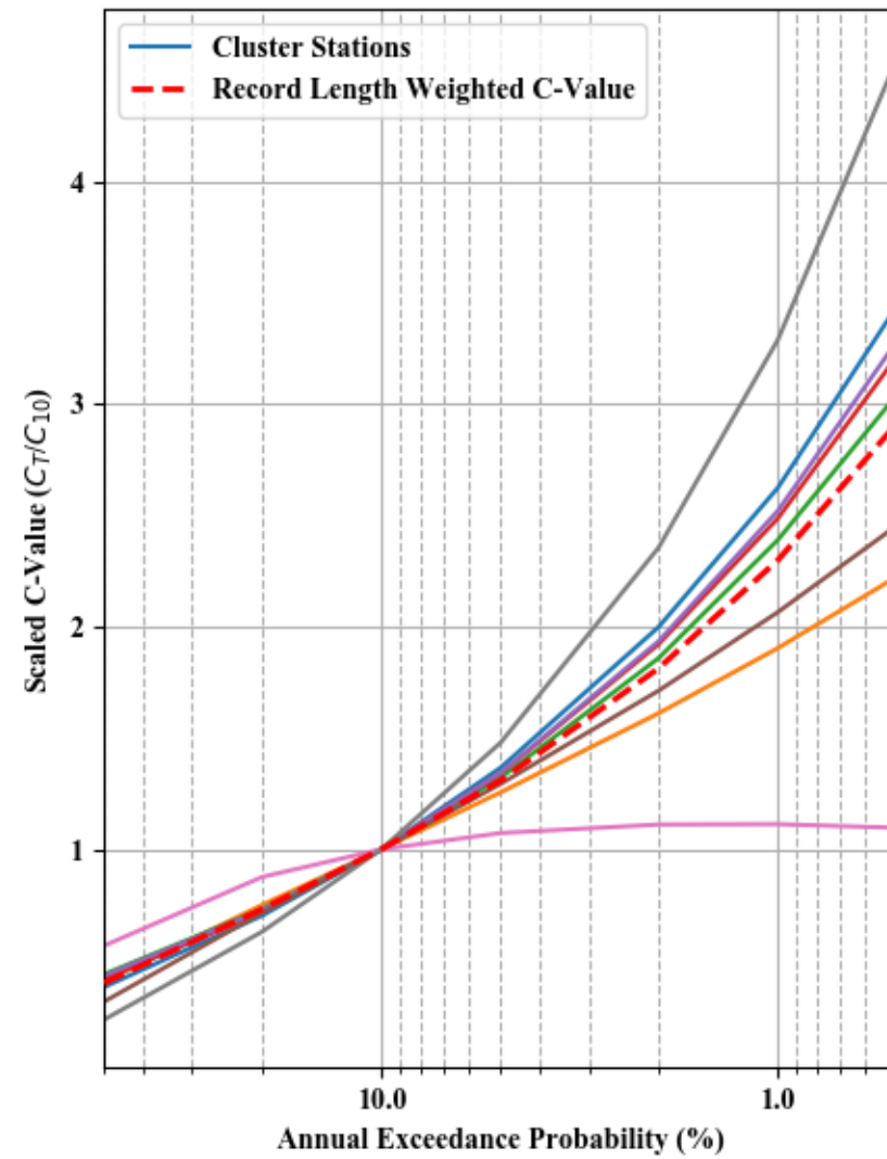
Dimensionless Peak Flow and Scaled C-value - Cluster 22
