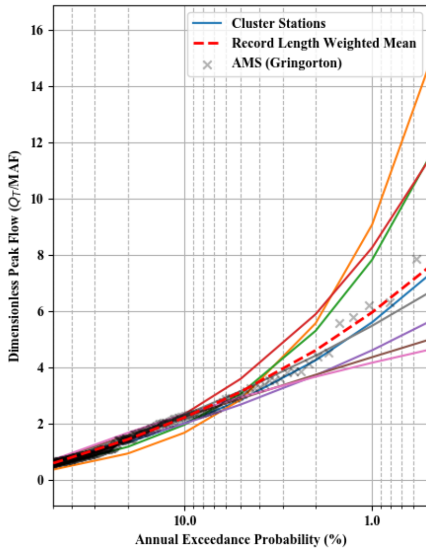
Dimensionless Peak Flow and Scaled C-value - Cluster 39
