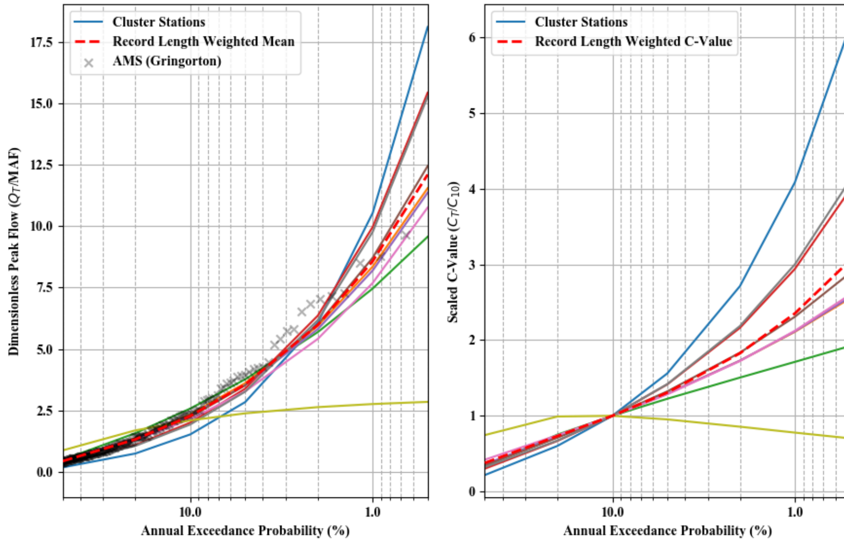
Dimensionless Peak Flow and Scaled C-value - Cluster 11
