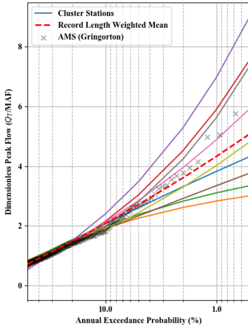
Dimensionless Peak Flow and Scaled C-value - Cluster 41
