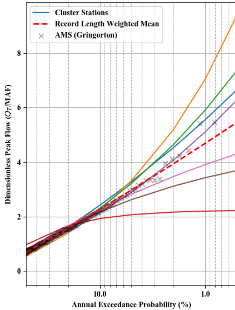
Dimensionless Peak Flow and Scaled C-value - Cluster 32
