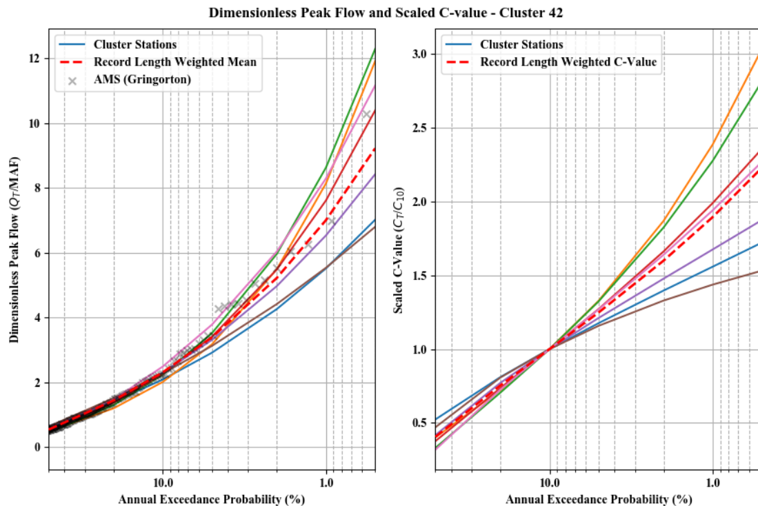
Figure 8.1 Dimensionless Peak flow (left) and Scaled C_T growth curves (right) for Cluster 42 indicating the record length weighted average curves (red dash) in relation to the sites within the cluster (coloured lines)
