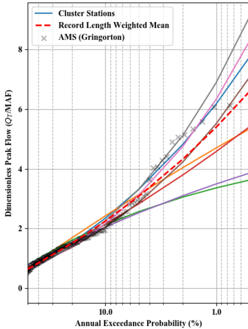
Dimensionless Peak Flow and Scaled C-value - Cluster 15
