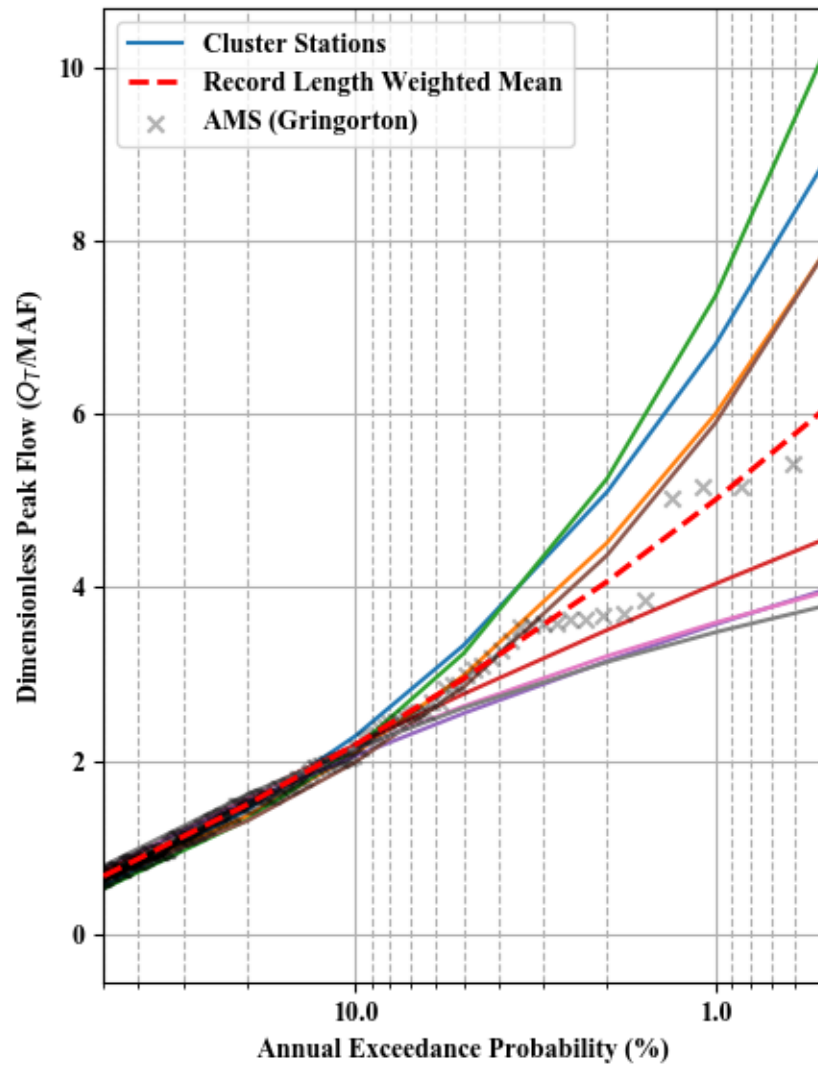
Dimensionless Peak Flow and Scaled C-value - Cluster 38
