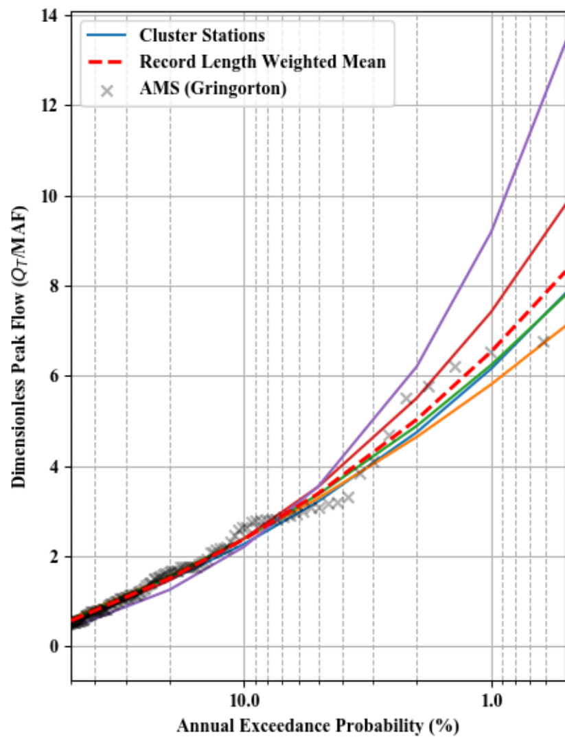
Dimensionless Peak Flow and Scaled C-value - Cluster 28
