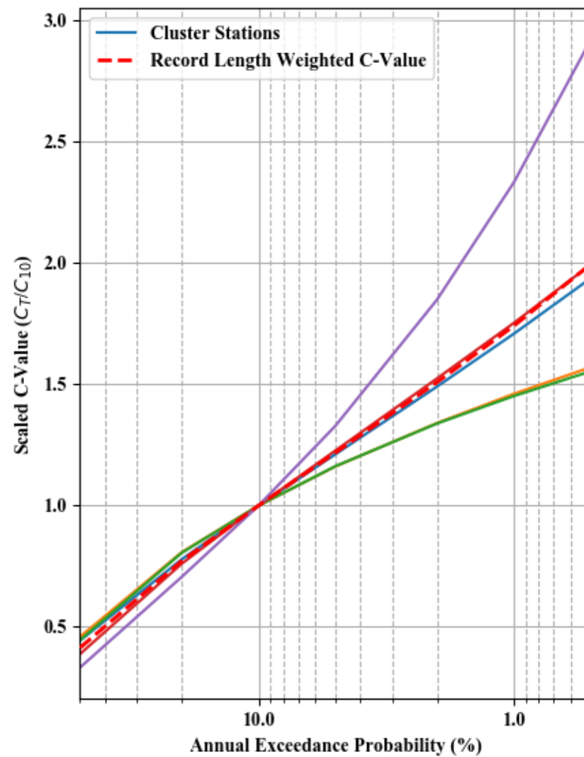
Dimensionless Peak Flow and Scaled C-value - Cluster 28
