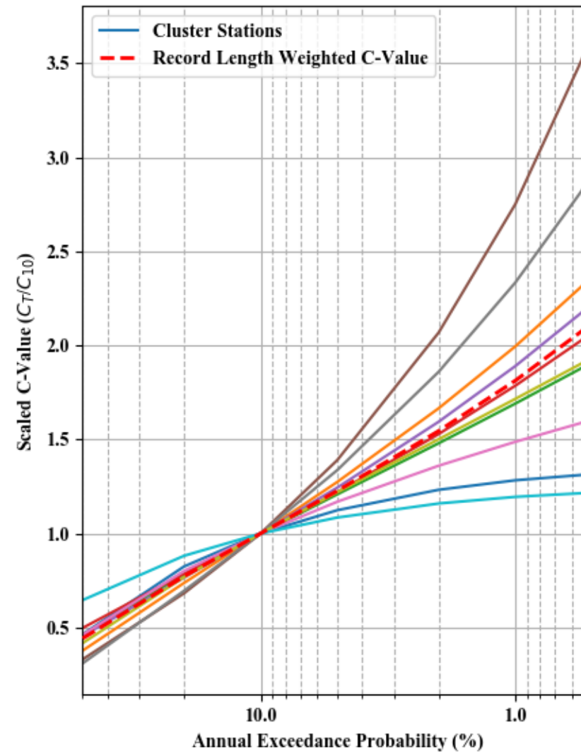
Dimensionless Peak Flow and Scaled C-value - Cluster 16
