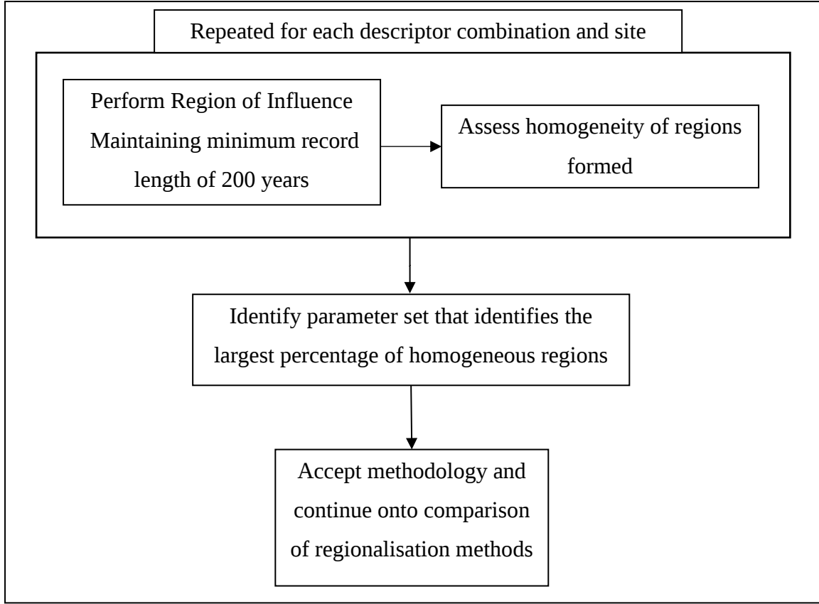
Figure 3.5 Region of Influence methodology flow diagram
