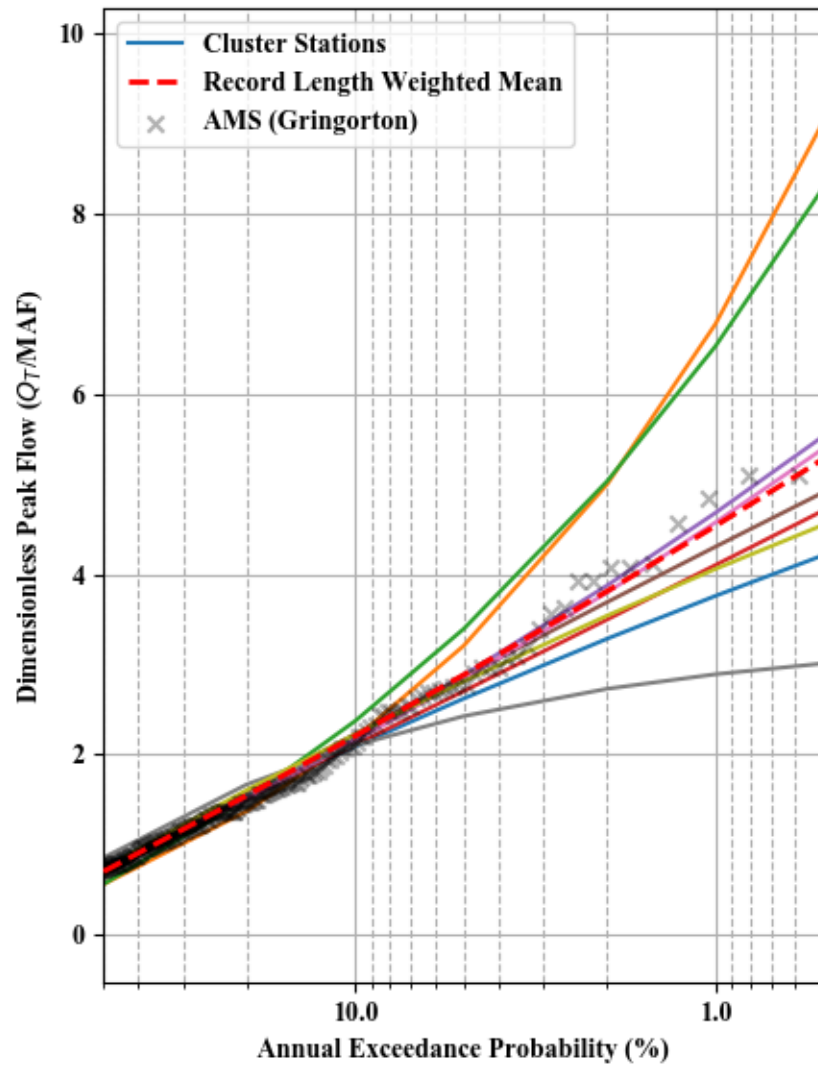
Dimensionless Peak Flow and Scaled C-value - Cluster 9
