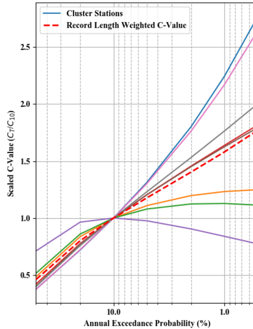
Dimensionless Peak Flow and Scaled C-value - Cluster 13
