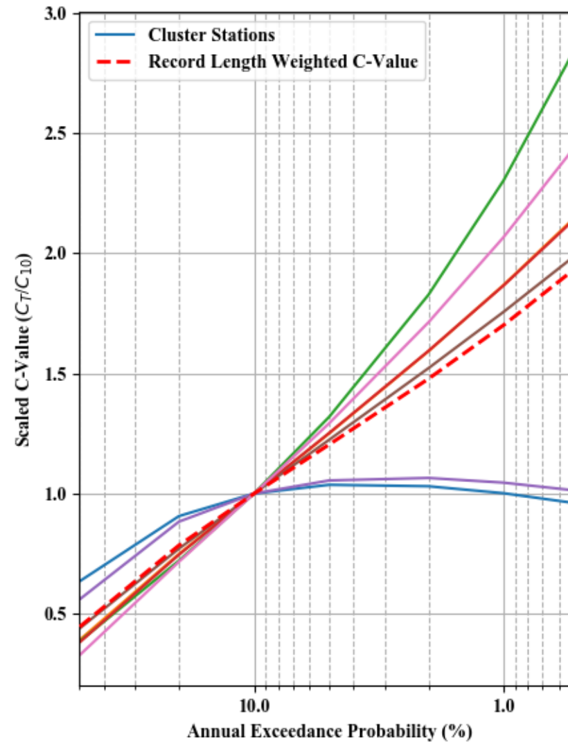
Dimensionless Peak Flow and Scaled C-value - Cluster 8
