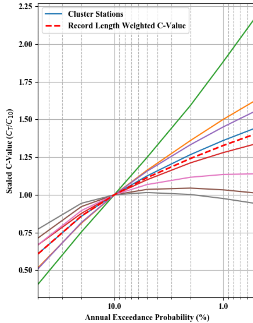
Dimensionless Peak Flow and Scaled C-value - Cluster 21
