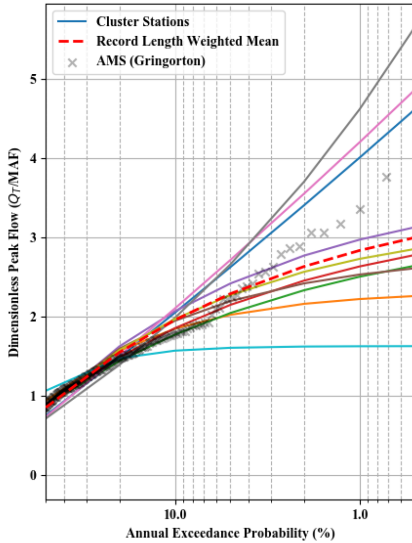
Dimensionless Peak Flow and Scaled C-value - Cluster 1
