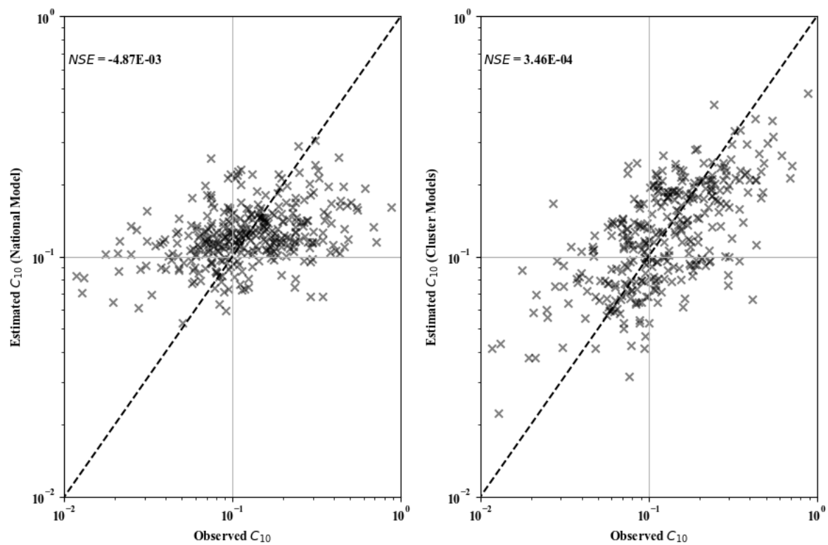
Figure 8.2 Observed versus estimated C_{10} for the national- (left) and cluster based (right) models
