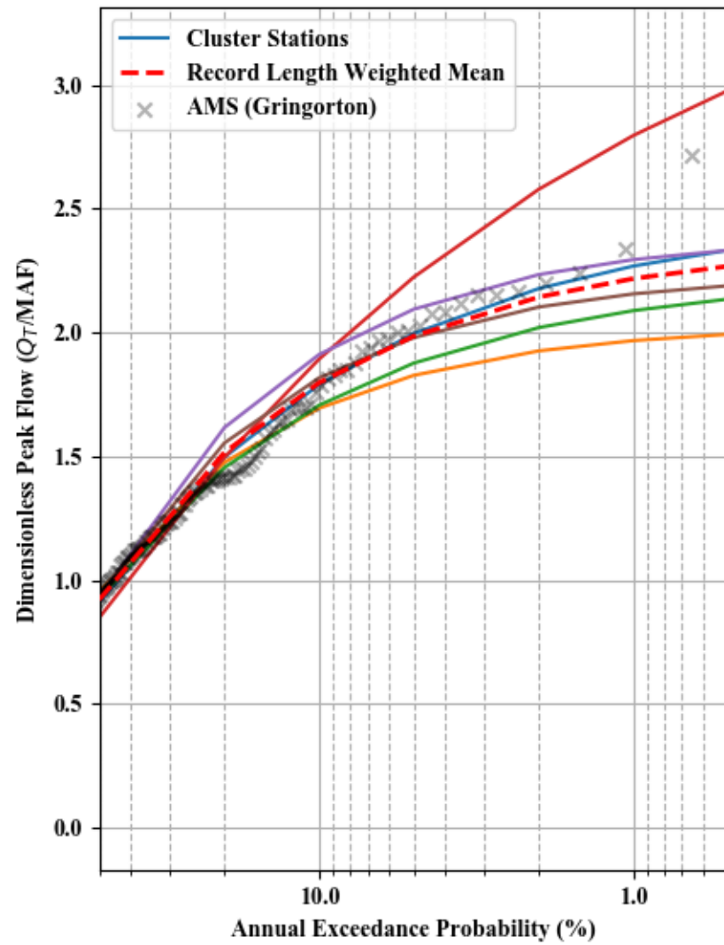
Dimensionless Peak Flow and Scaled C-value - Cluster 20
