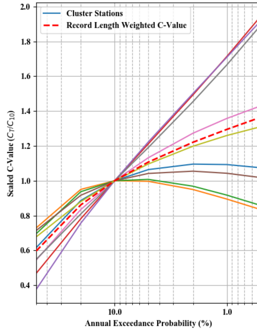
Dimensionless Peak Flow and Scaled C-value - Cluster 41
