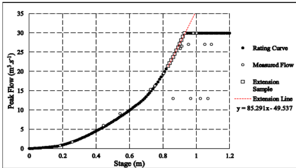
Figure 3.1 Example of a rating curve exceedance and extension the adopted extension methodology
