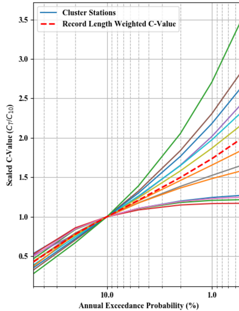
Dimensionless Peak Flow and Scaled C-value - Cluster 25
