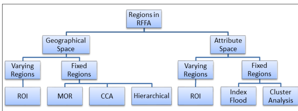
Figure 2.1 RFFA methods used in the formation of regions (after Rahman et al. 2012)
