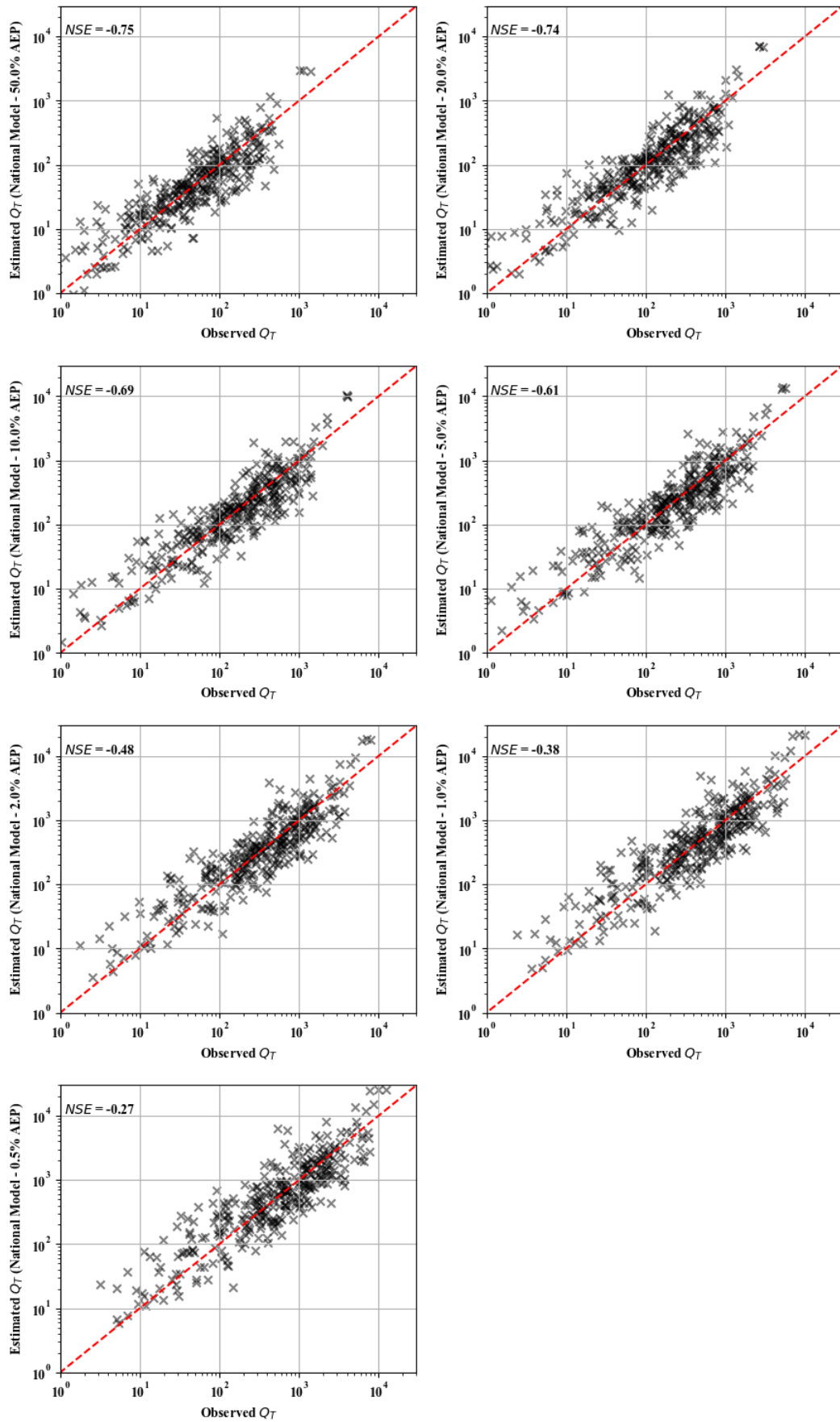
Figure 8.4 Estimated vs observed Q_T using the C_T National based approach for the 50, 20, 10, 5, 2, 1 and 0.5% annual exceedance probabilities
