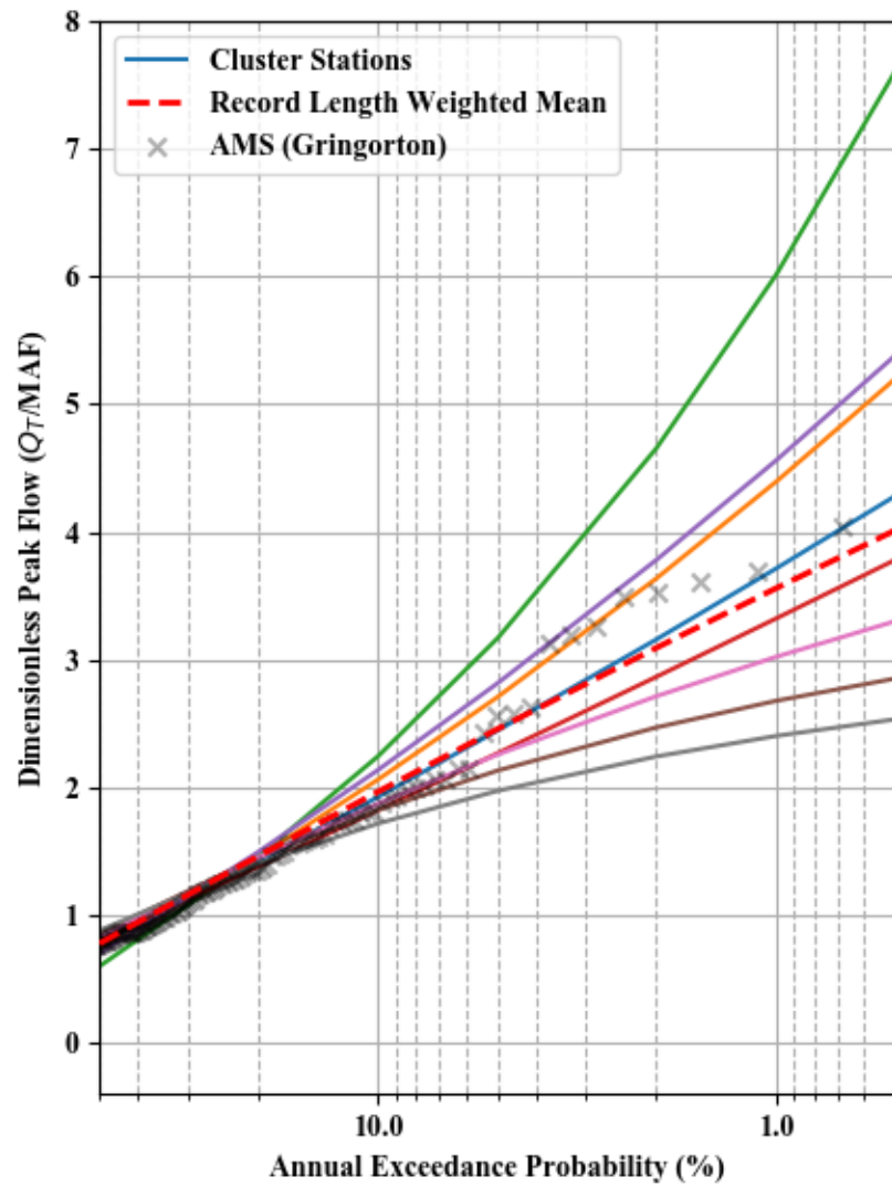
Dimensionless Peak Flow and Scaled C-value - Cluster 21
