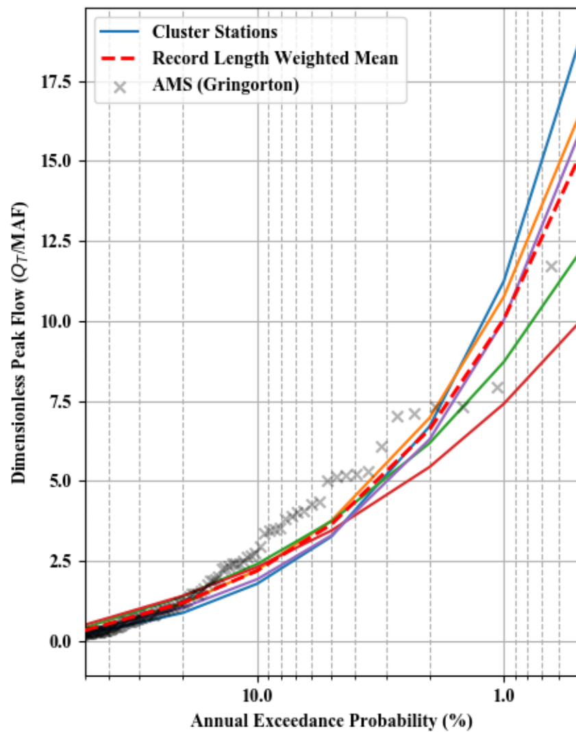
Dimensionless Peak Flow and Scaled C-value - Cluster 30
