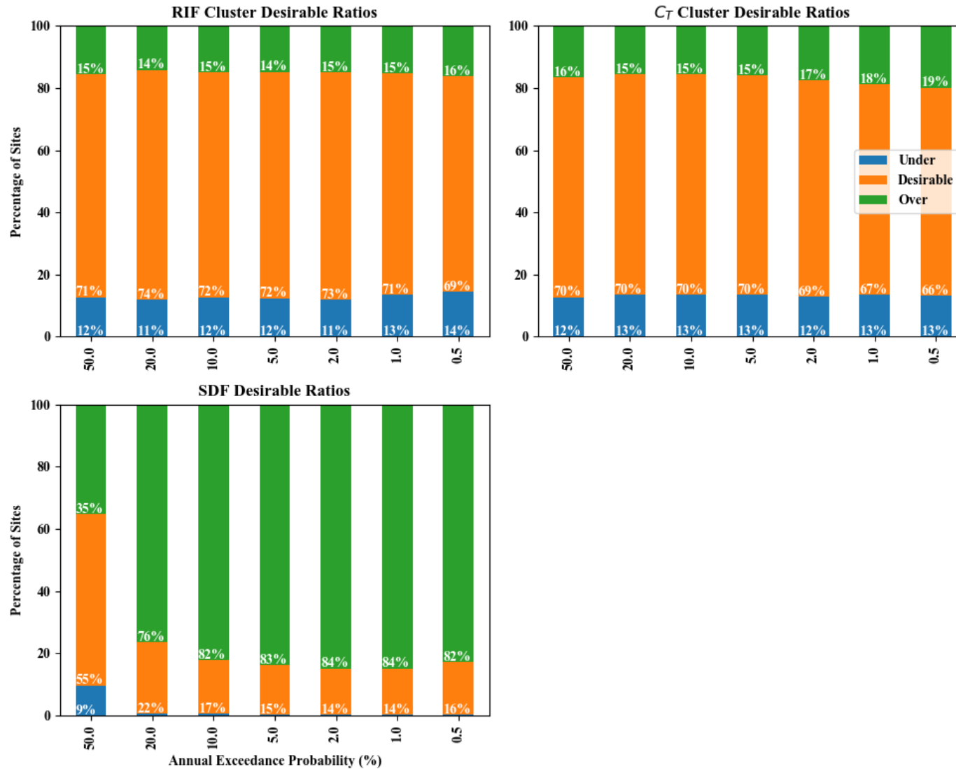
Figure 8.11 Comparison of the percentage of Q_T estimates within the desirable ratio defined by Rahman et al. (2012), between the RIF (top left), C_T (top right) and the SDF (bottom left) approaches
