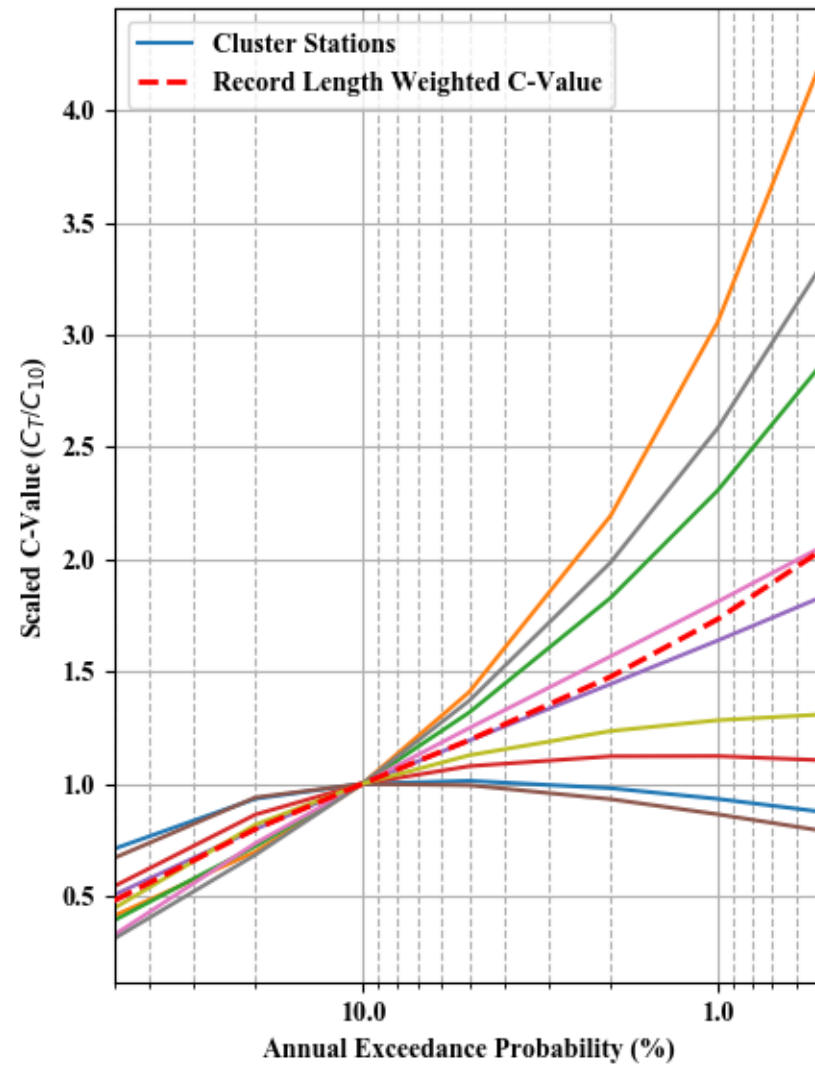
Dimensionless Peak Flow and Scaled C-value - Cluster 34
