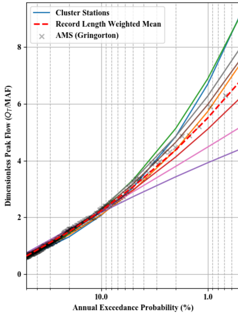
Dimensionless Peak Flow and Scaled C-value - Cluster 31
