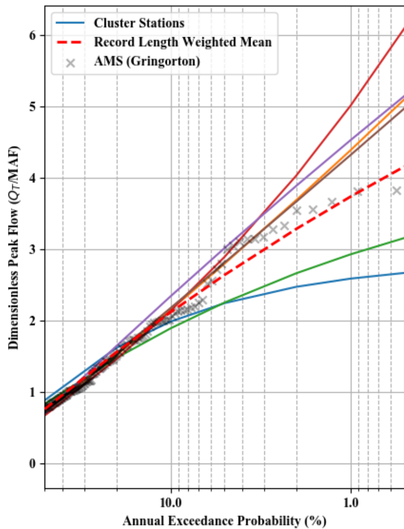
Dimensionless Peak Flow and Scaled C-value - Cluster 27
