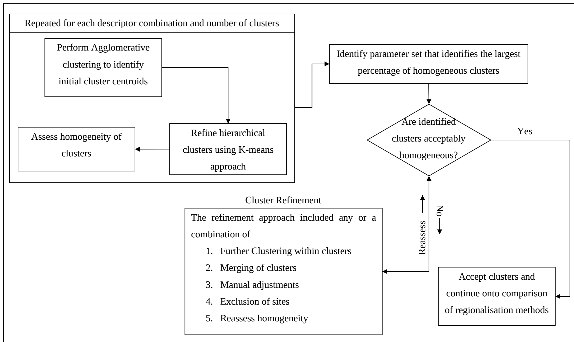
Figure 3.4 Clustering methodology flow diagram
