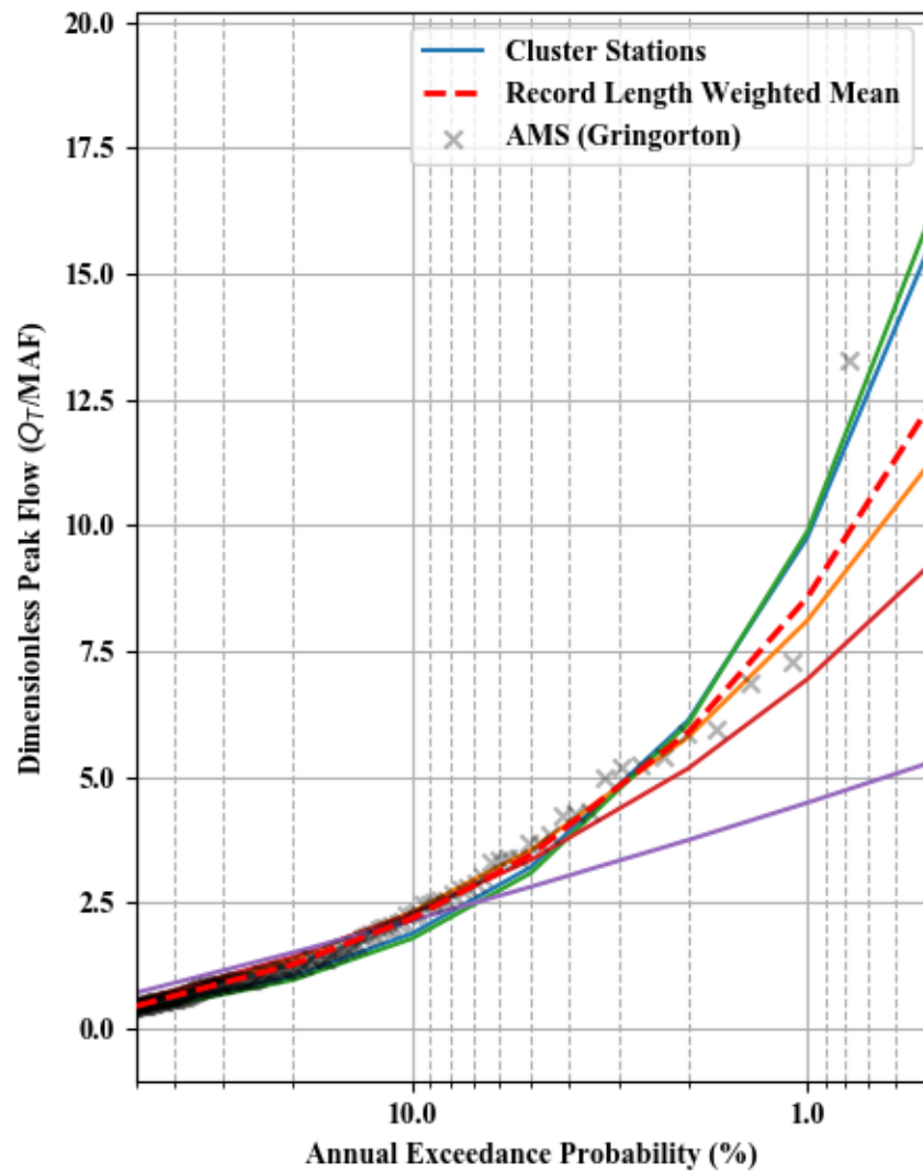
Dimensionless Peak Flow and Scaled C-value - Cluster 3
