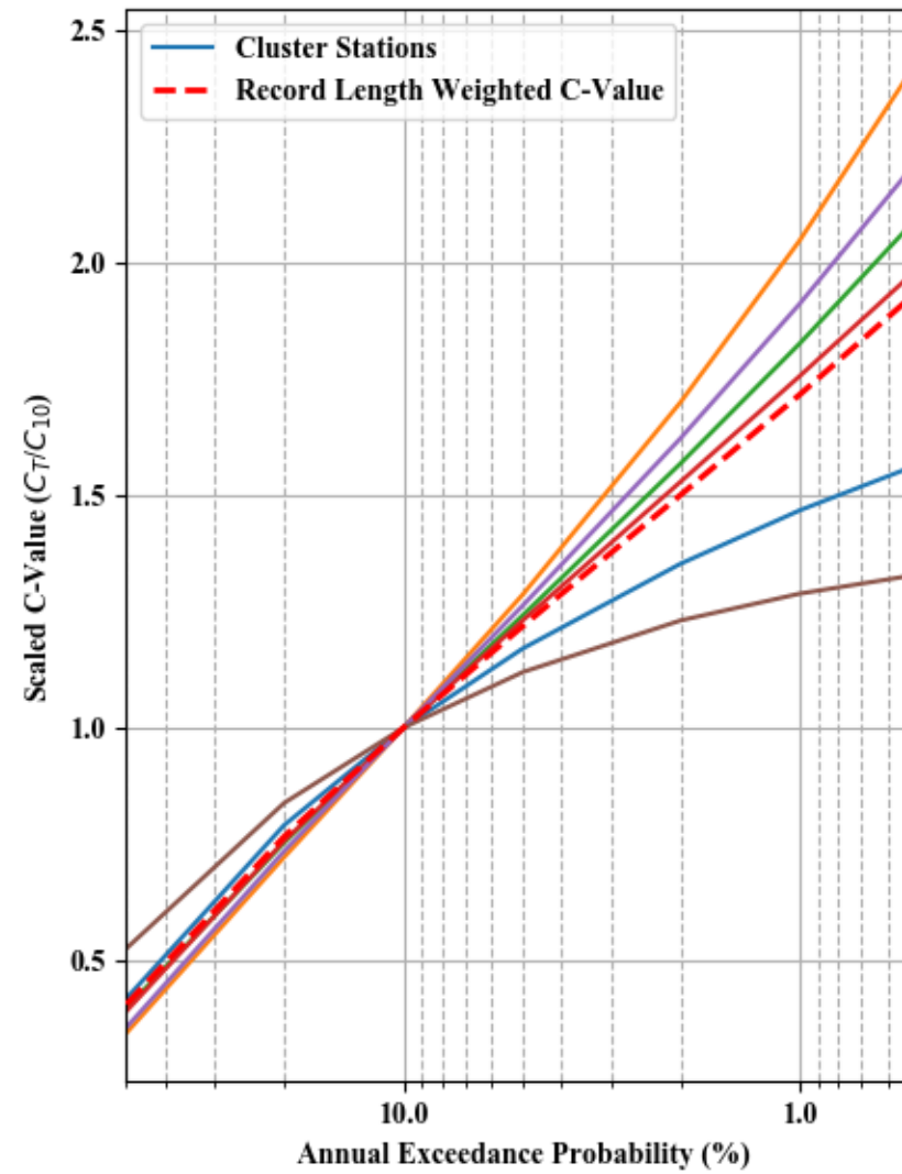
Dimensionless Peak Flow and Scaled C-value - Cluster 6
