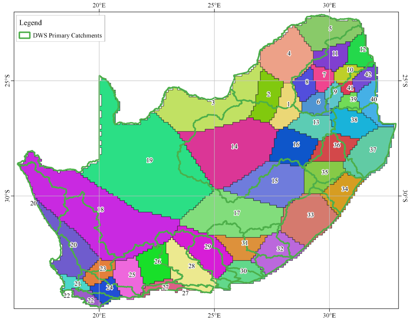
Figure 7.2 Delineation of national cluster association based on location and distance in relation to the DWS primary drainage regions (green) from the sea at a scale of 0.1 degrees
