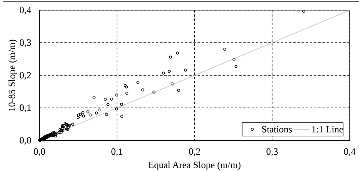
Figure 4.2 Average slope comparison
