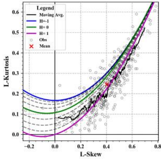
Figure 6.1 L-moment ratio diagram for all 383 selected sites using untransformed data indicating the KAPPA distribution h value contours at 0.25 intervals and the record length weighted mean L-skew and L-kurtosis.
