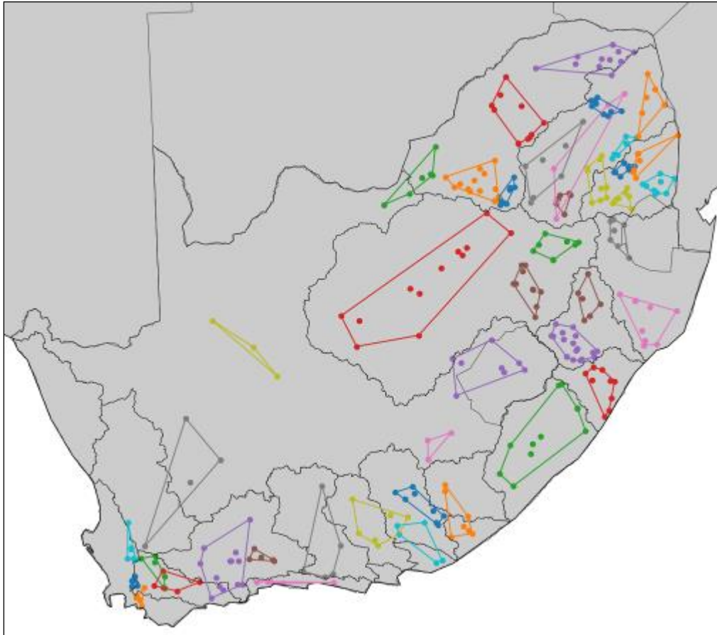
Figure 7.1 Distribution of the 42 relatively homogeneous clusters identified
