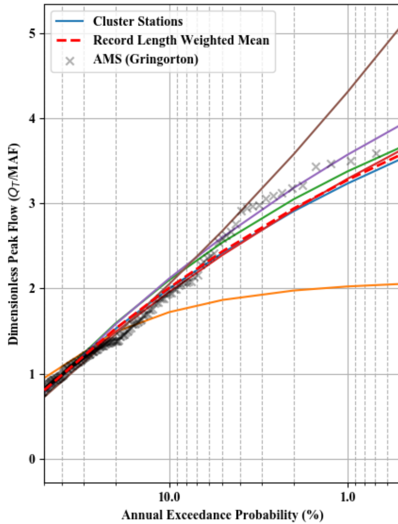
Dimensionless Peak Flow and Scaled C-value - Cluster 36
