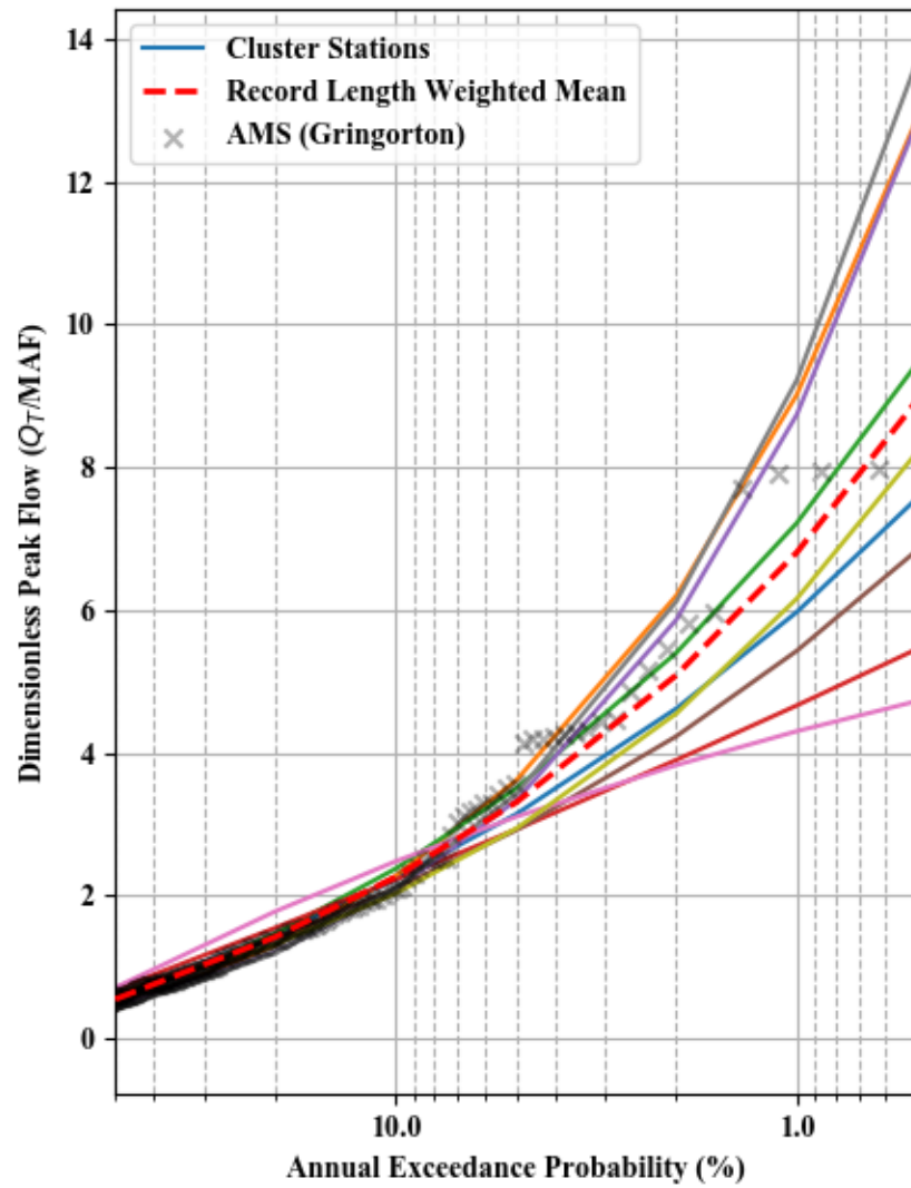
Dimensionless Peak Flow and Scaled C-value - Cluster 40
