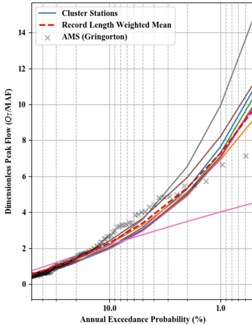
Dimensionless Peak Flow and Scaled C-value - Cluster 22
