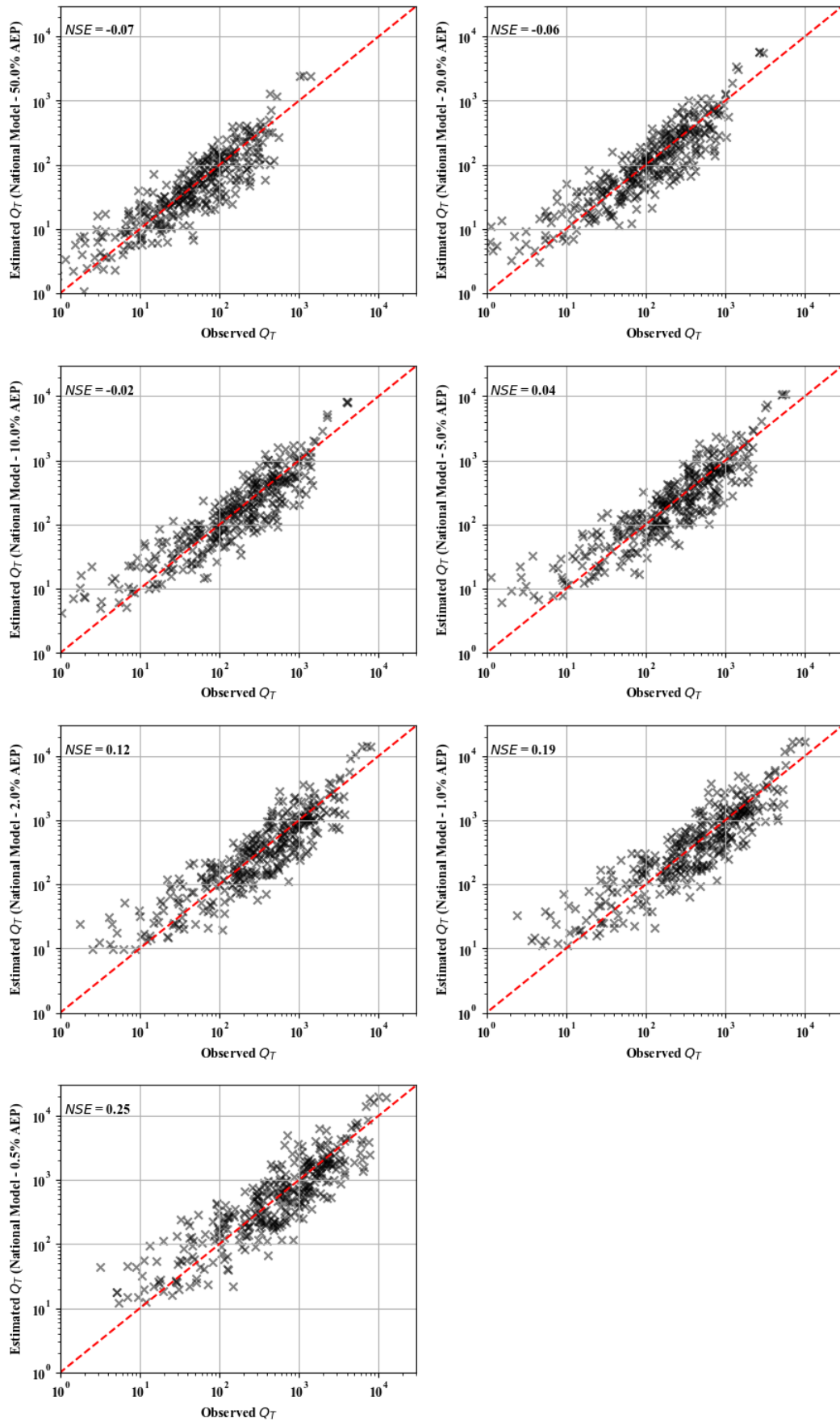
Figure 8.6 Estimated vs observed Q_T using the RIF National based approach for the 50, 20, 10, 5, 2, 1 and 0.5% annual exceedance probabilities
