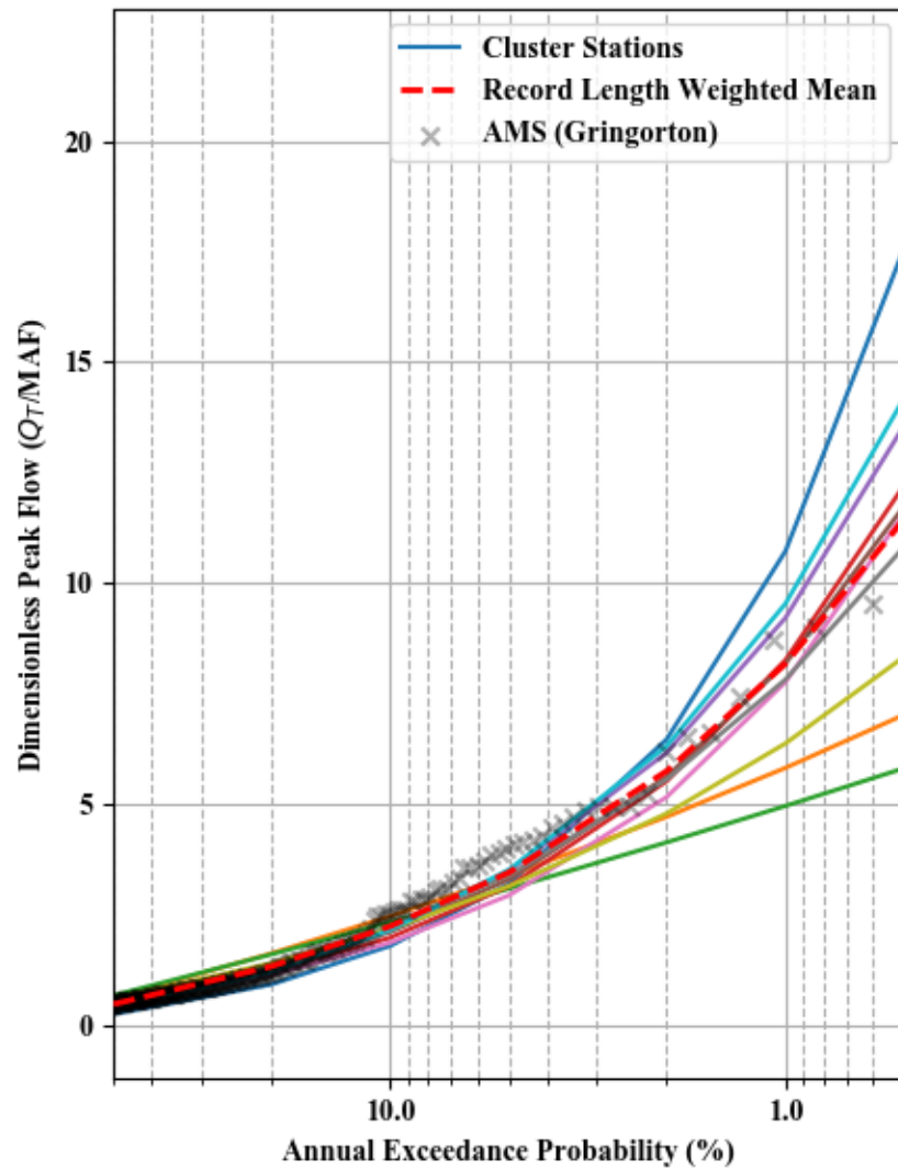
Dimensionless Peak Flow and Scaled C-value - Cluster 37
