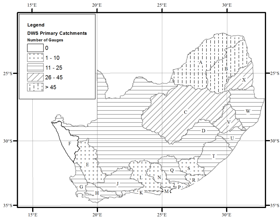
Figure 5.2 Number of gauging stations per DWS primary drainage region across South Africa
