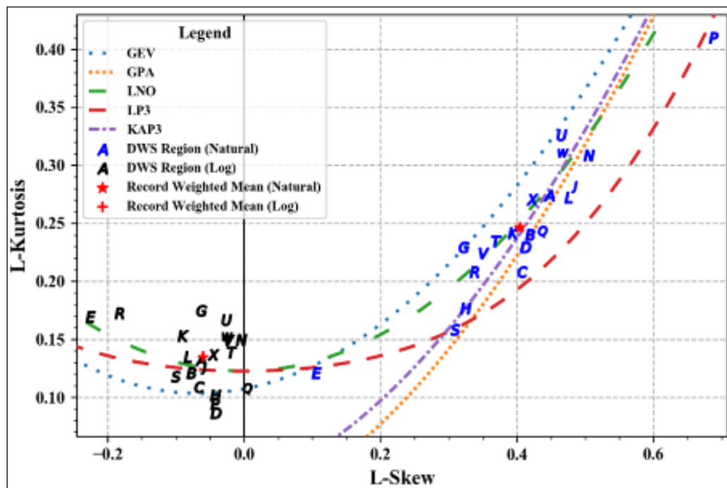
Figure 6.3 L-moment ratio diagram indicating the position of the record length weighted mean L-skew and L-kurtosis per DWS drainage region, represented by the relevant alphabetic numeral, for natural (blue) and log transformed (black) data as well as the record length weighted means of the entire dataset
