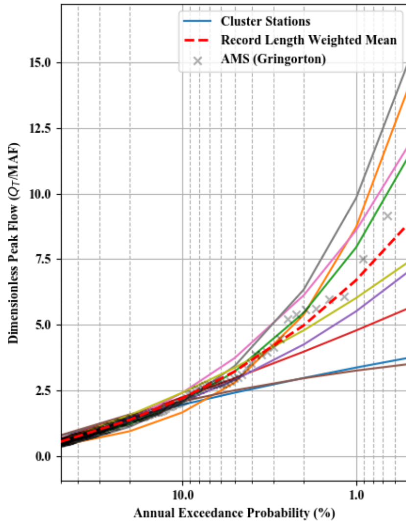
Dimensionless Peak Flow and Scaled C-value - Cluster 34
