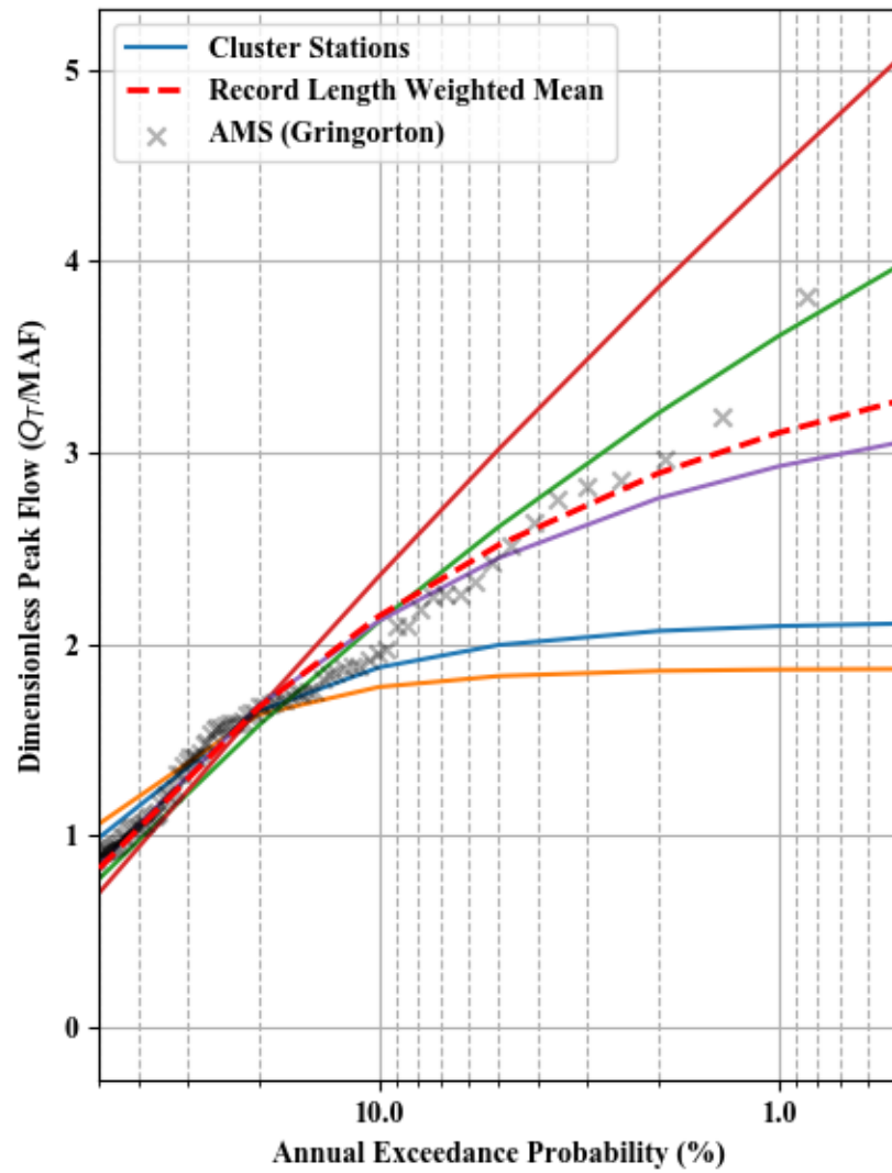
Dimensionless Peak Flow and Scaled C-value - Cluster 7
