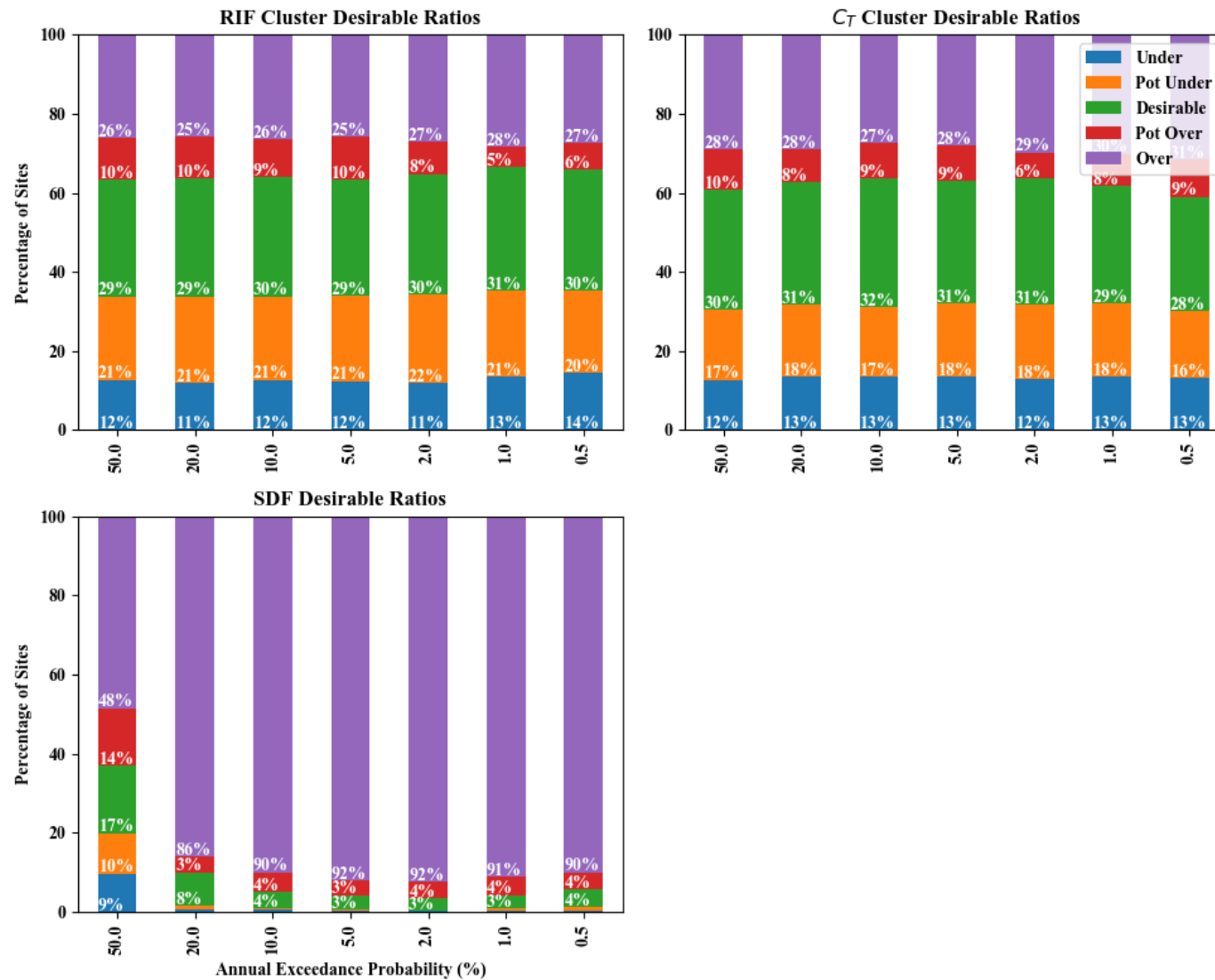
Figure 8.12 Comparison of the percentage of Q_T estimates within the desirable ratio defined by Naidoo (In Preparation), between the RIF (top left), C_T (top right) and the SDF (bottom left) approaches
