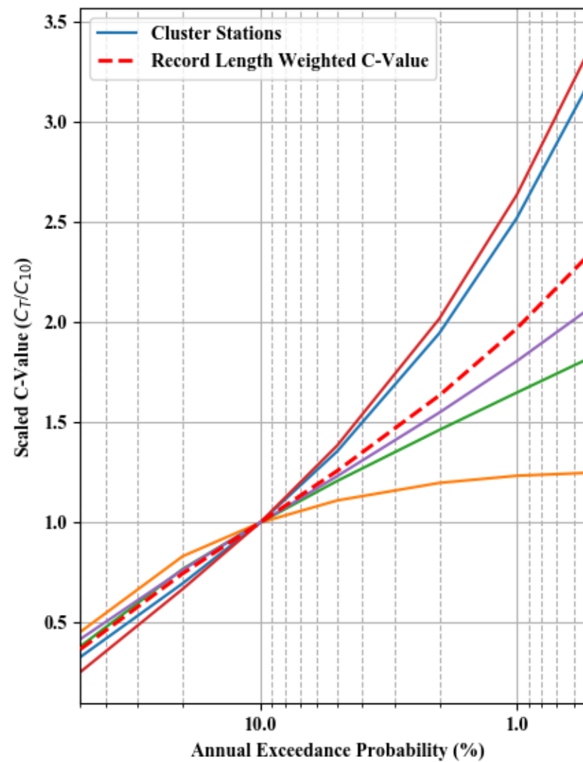
Dimensionless Peak Flow and Scaled C-value - Cluster 26
