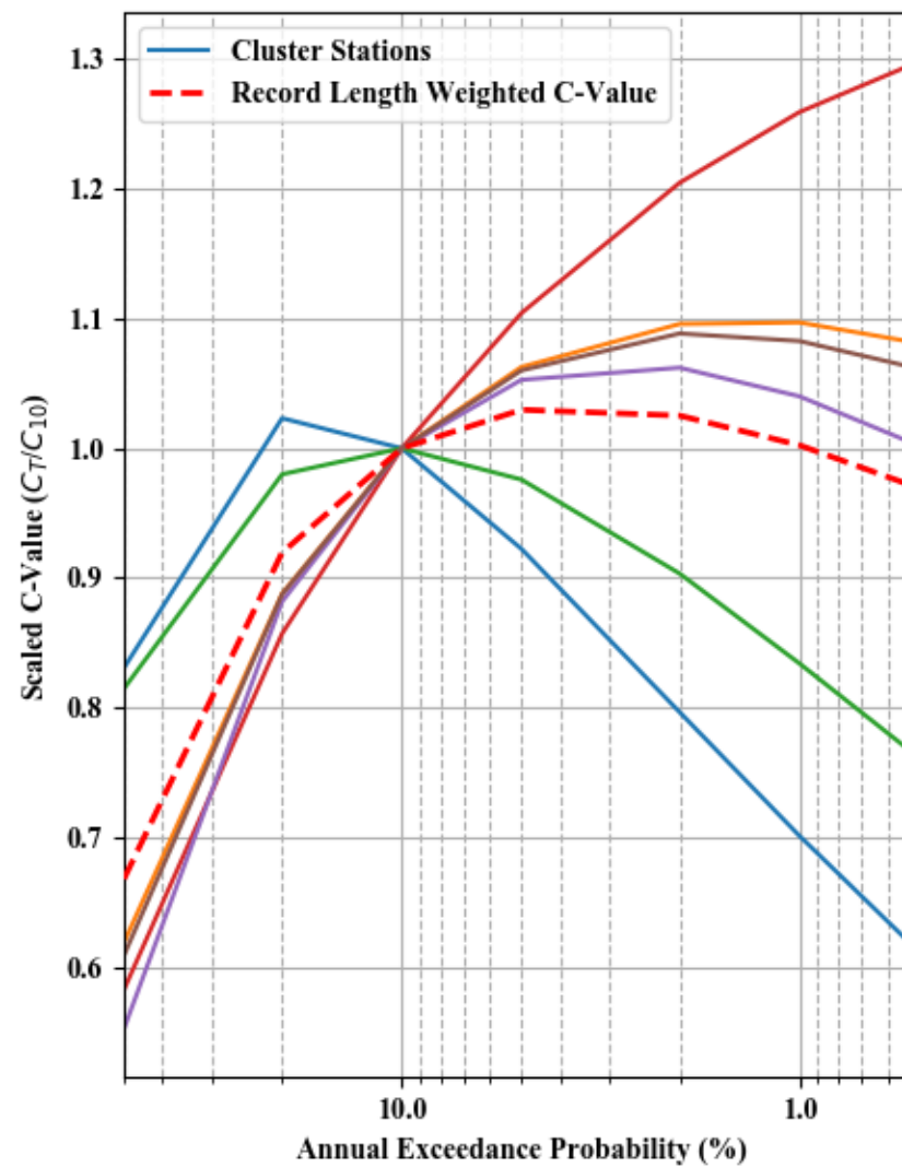
Dimensionless Peak Flow and Scaled C-value - Cluster 27
