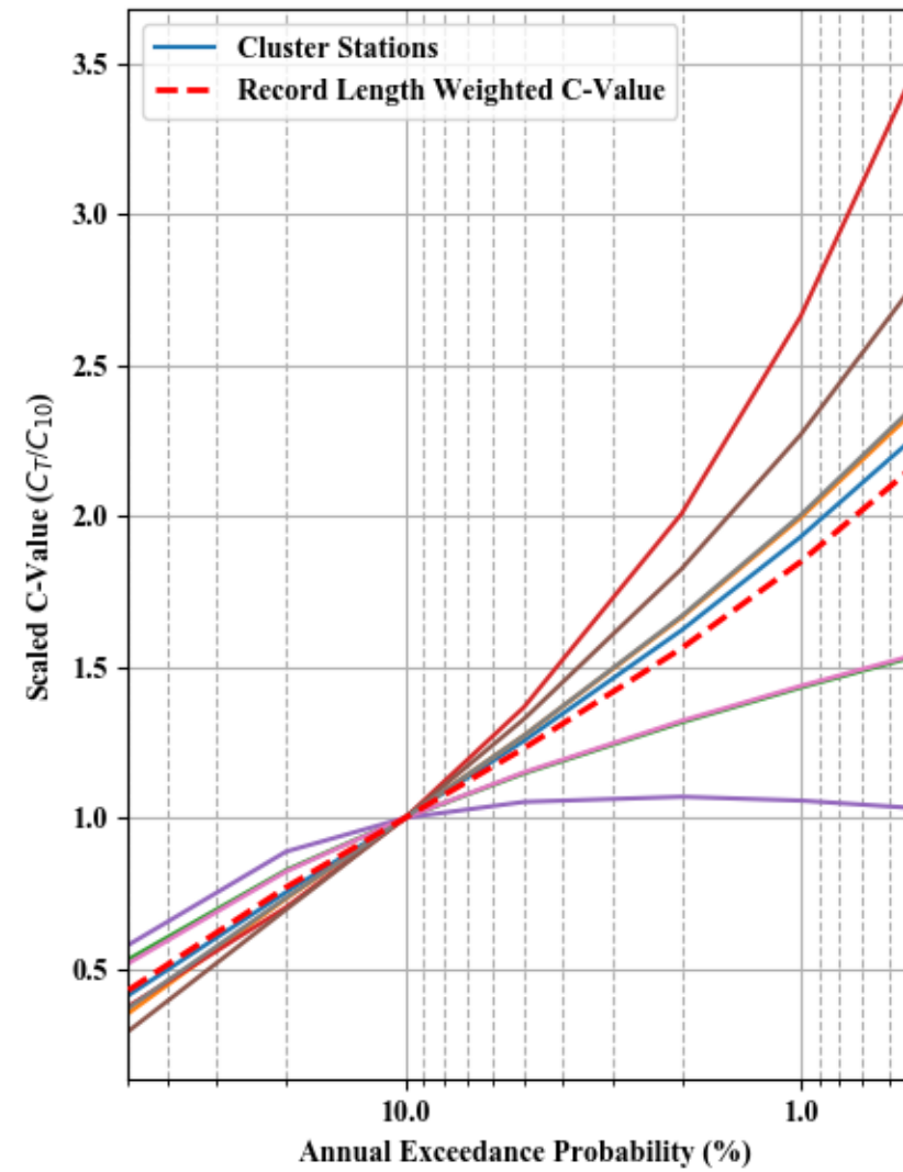
Dimensionless Peak Flow and Scaled C-value - Cluster 29
