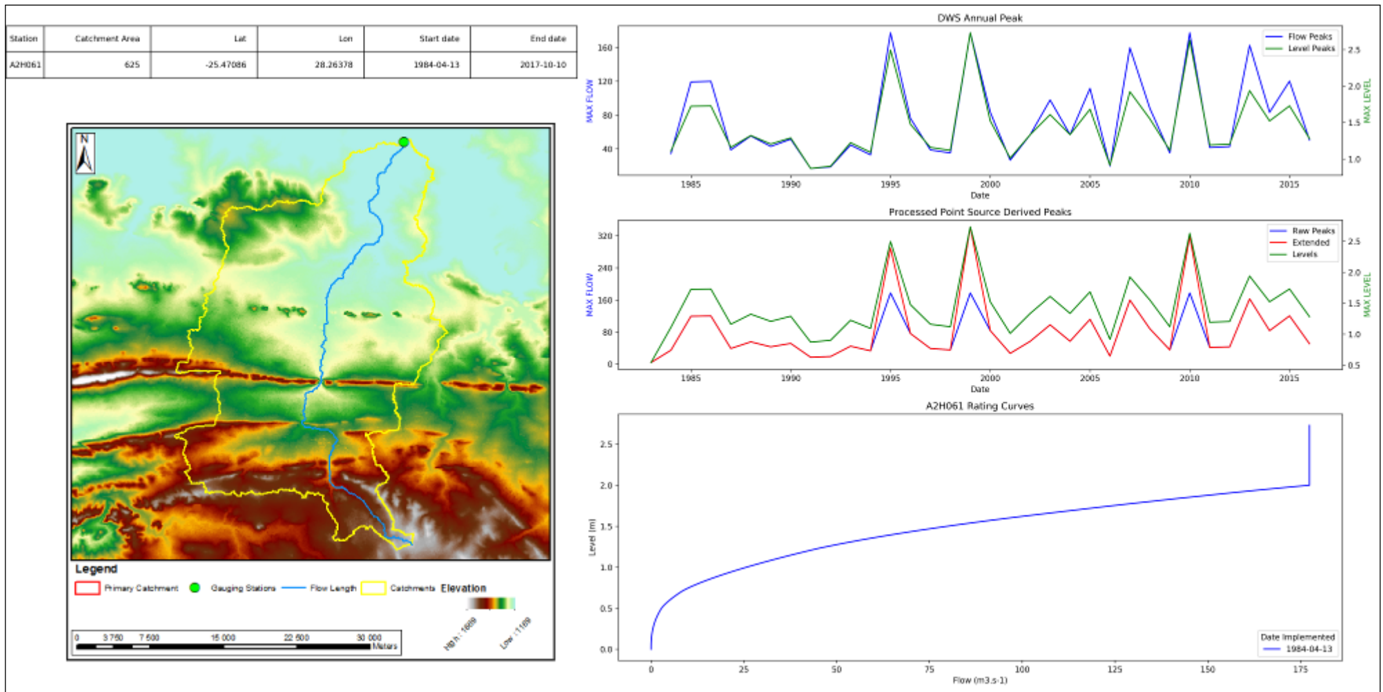
Figure 5.4 Catchment information for Gauging Station A2H061
