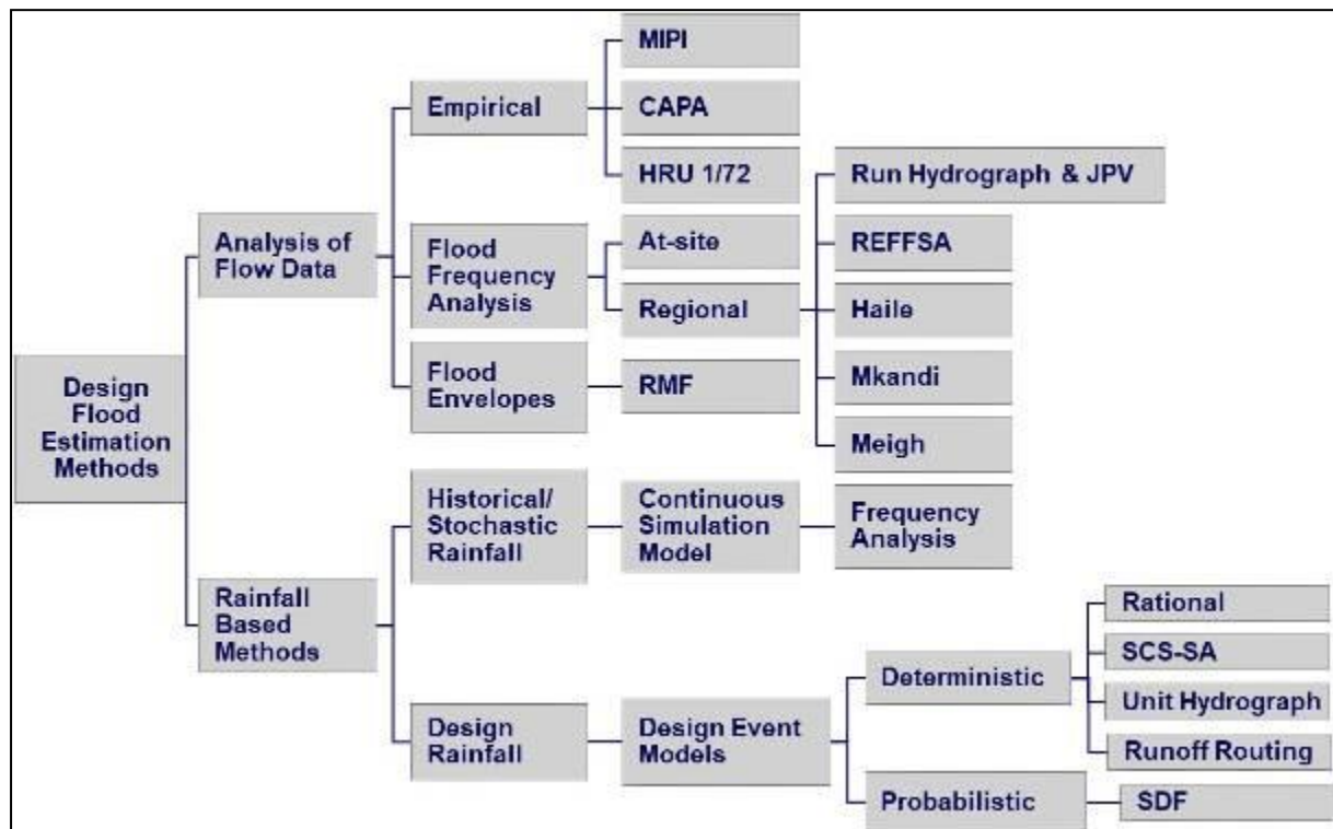
Figure 1.1 Design flood estimation methods (after Smithers 2012)
