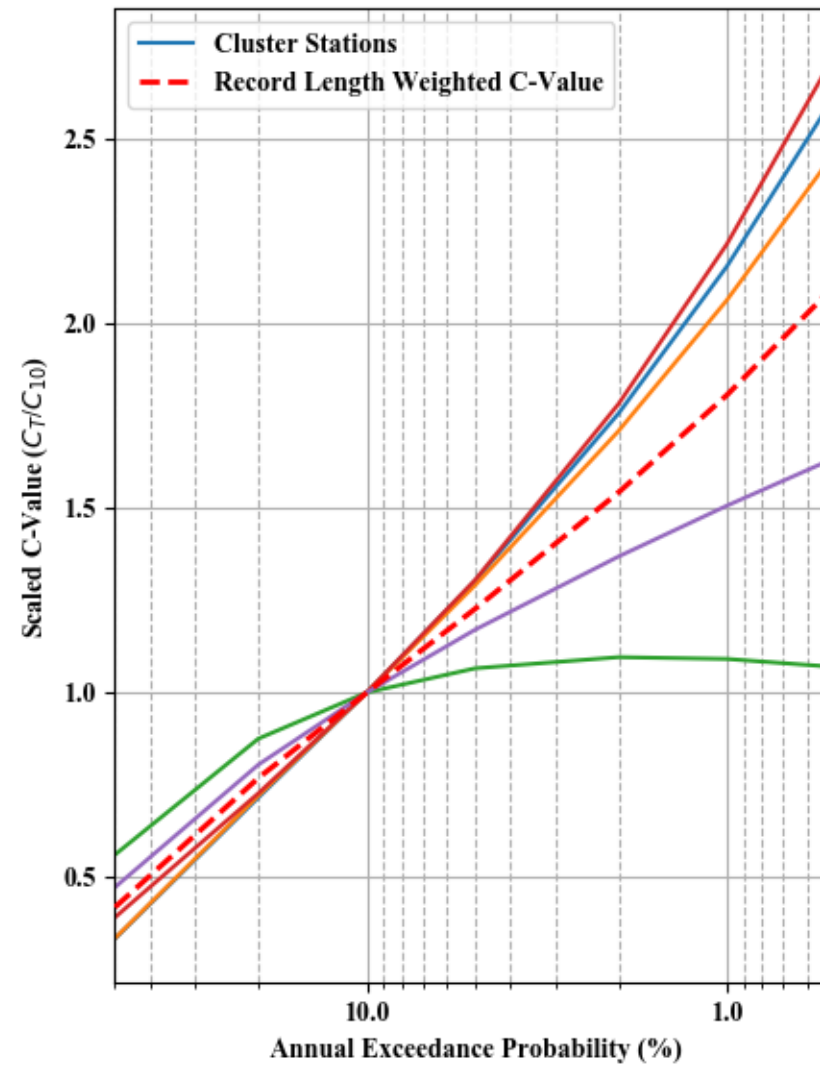
Dimensionless Peak Flow and Scaled C-value - Cluster 24
