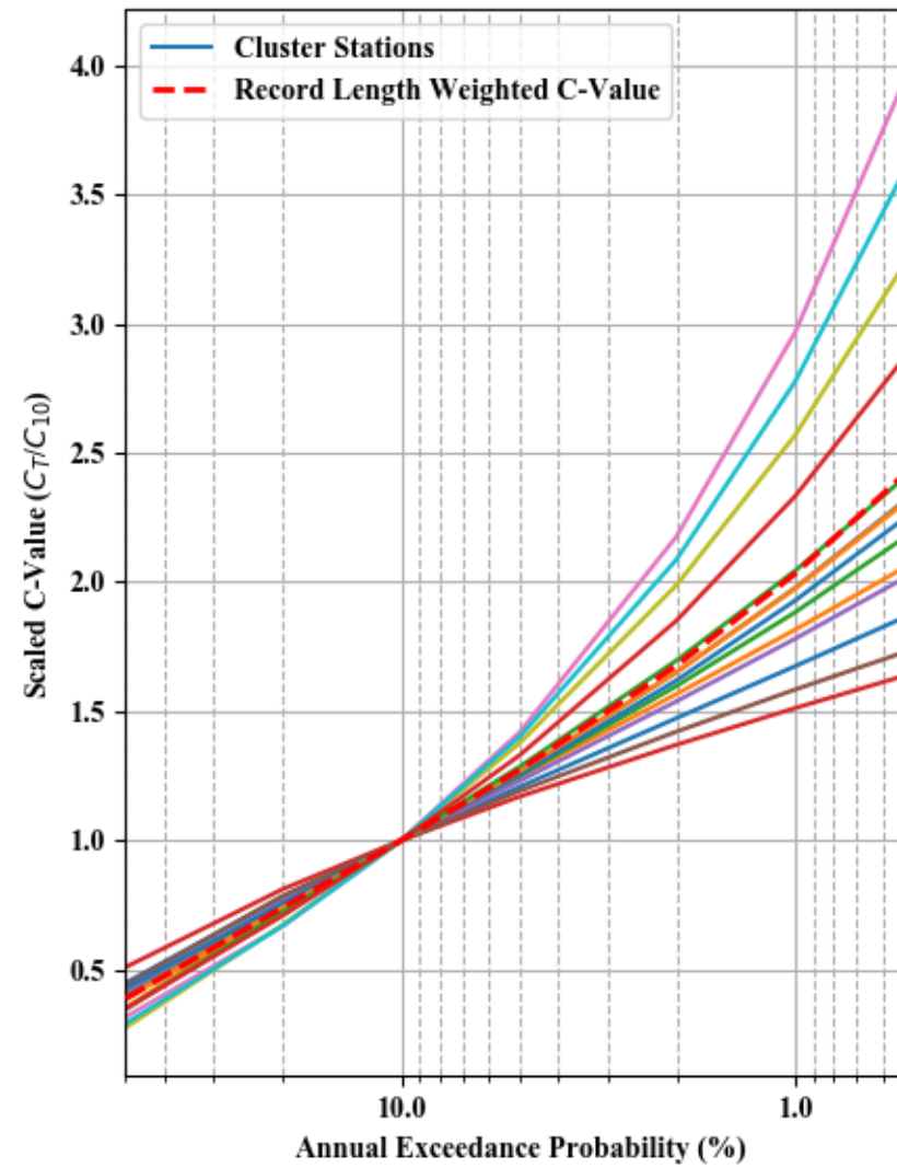
Dimensionless Peak Flow and Scaled C-value - Cluster 2
