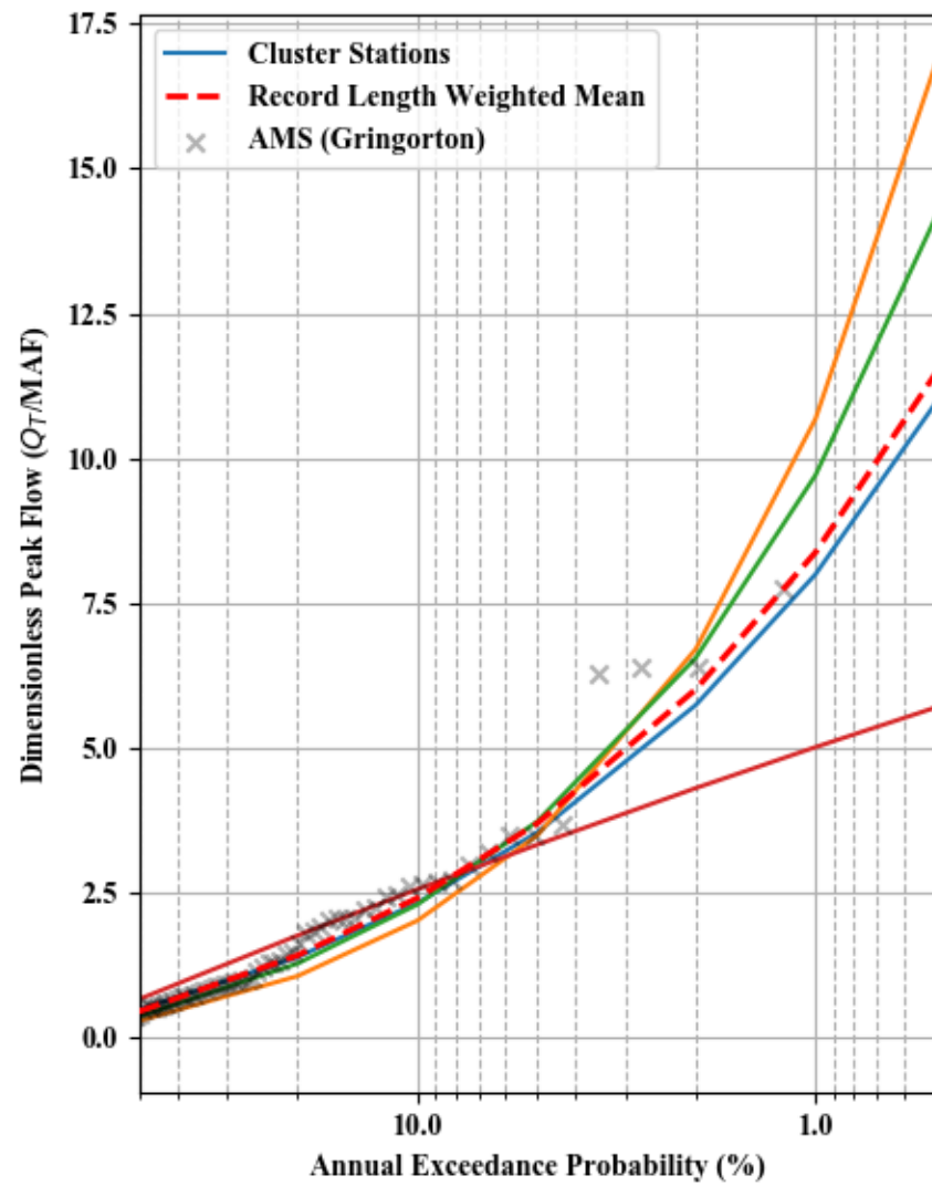
Dimensionless Peak Flow and Scaled C-value - Cluster 18
