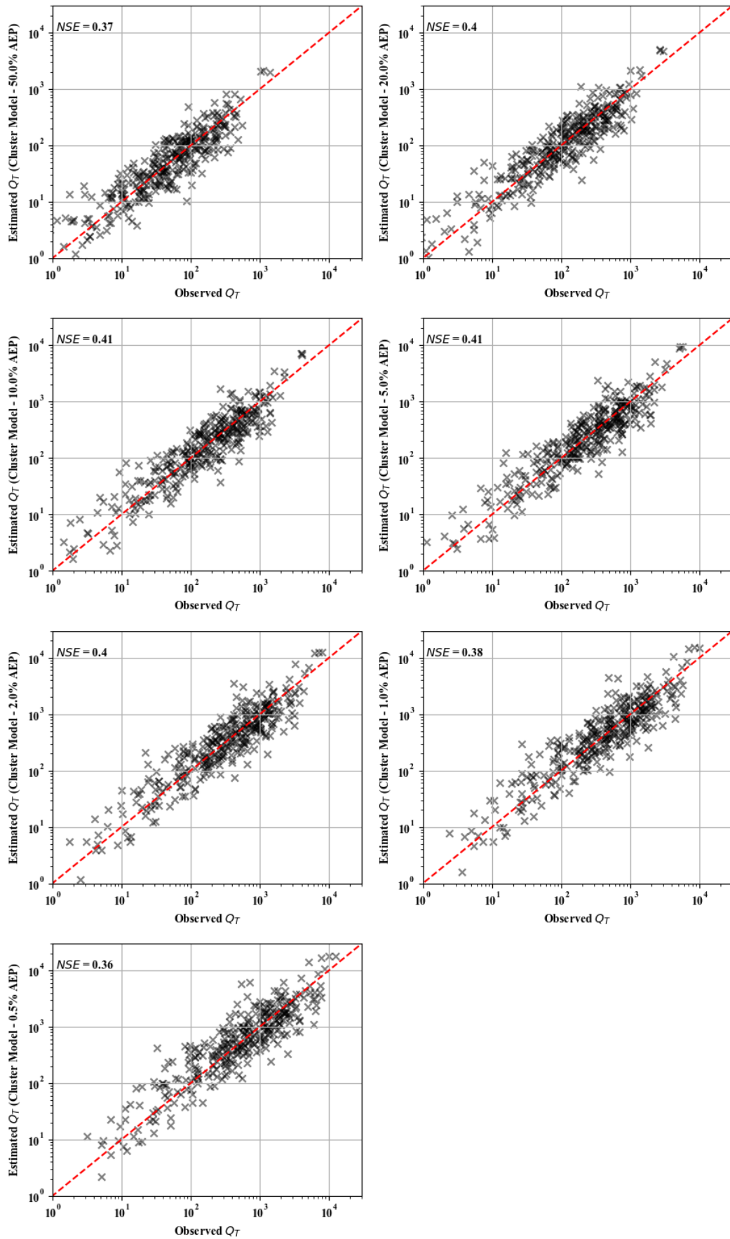
Figure 8.5 Estimated vs observed Q_T using the C_T Cluster based approach for the 50, 20, 10, 5, 2, 1 and 0.5% annual exceedance probabilities
