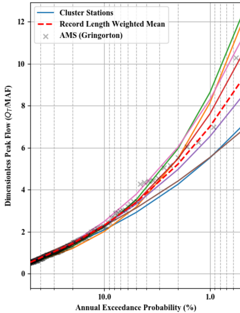
Dimensionless Peak Flow and Scaled C-value - Cluster 42
