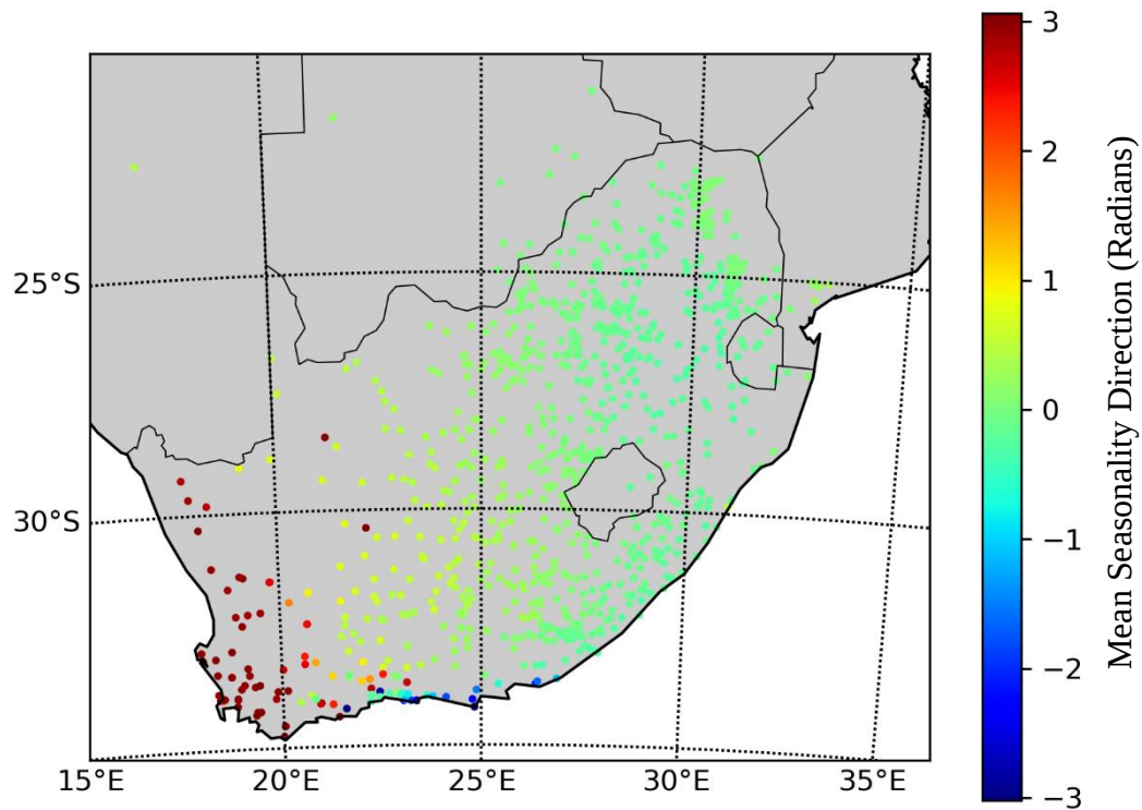
Figure 4.4 National rainfall seasonality indicating the mean direction (radians) of each site investigated
