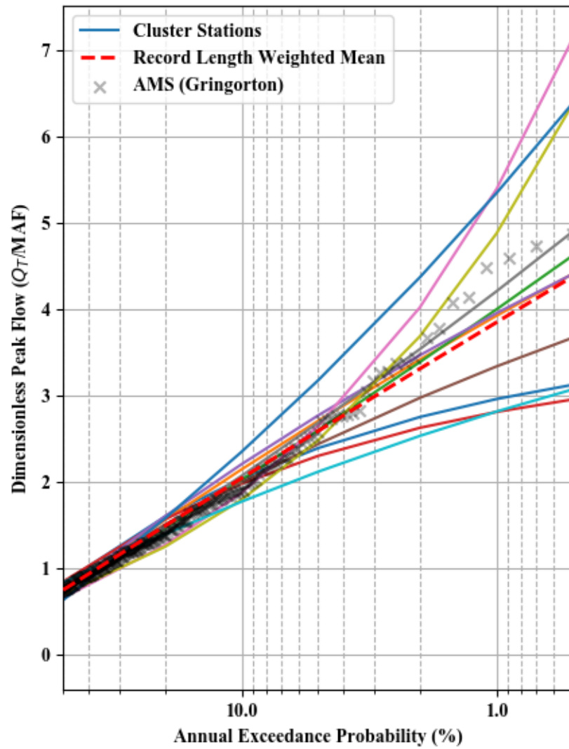
Dimensionless Peak Flow and Scaled C-value - Cluster 33
