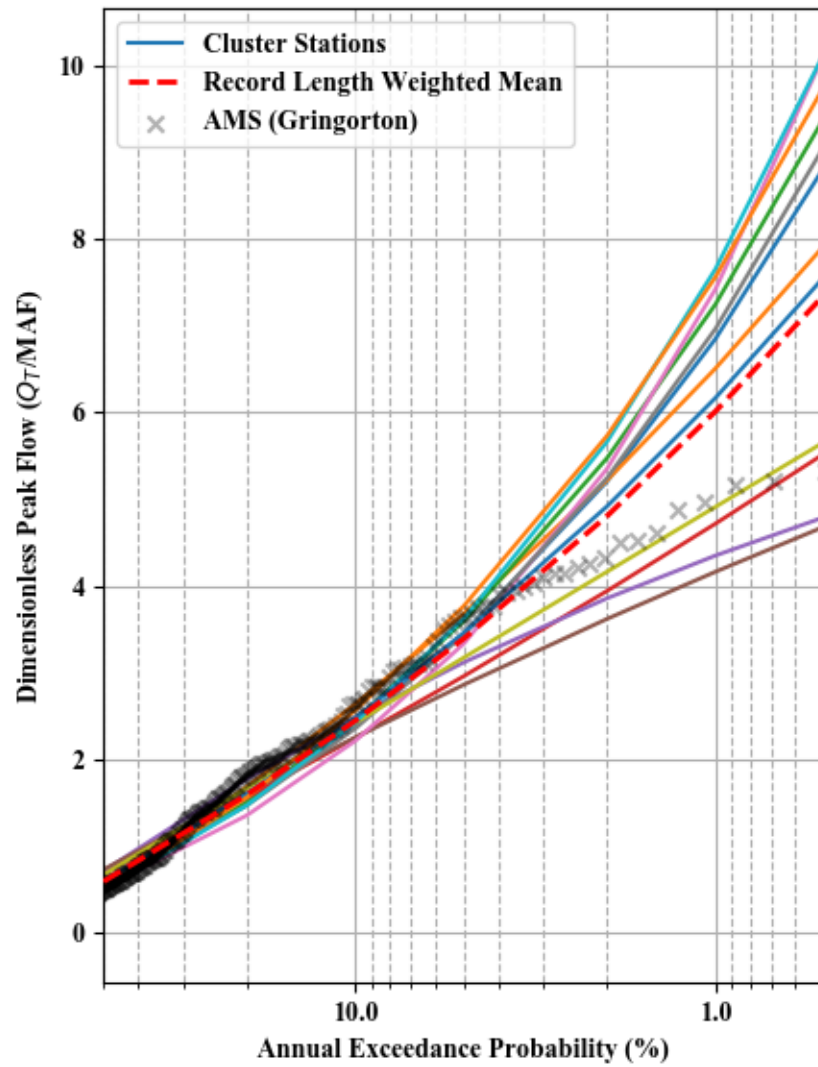
Dimensionless Peak Flow and Scaled C-value - Cluster 14
