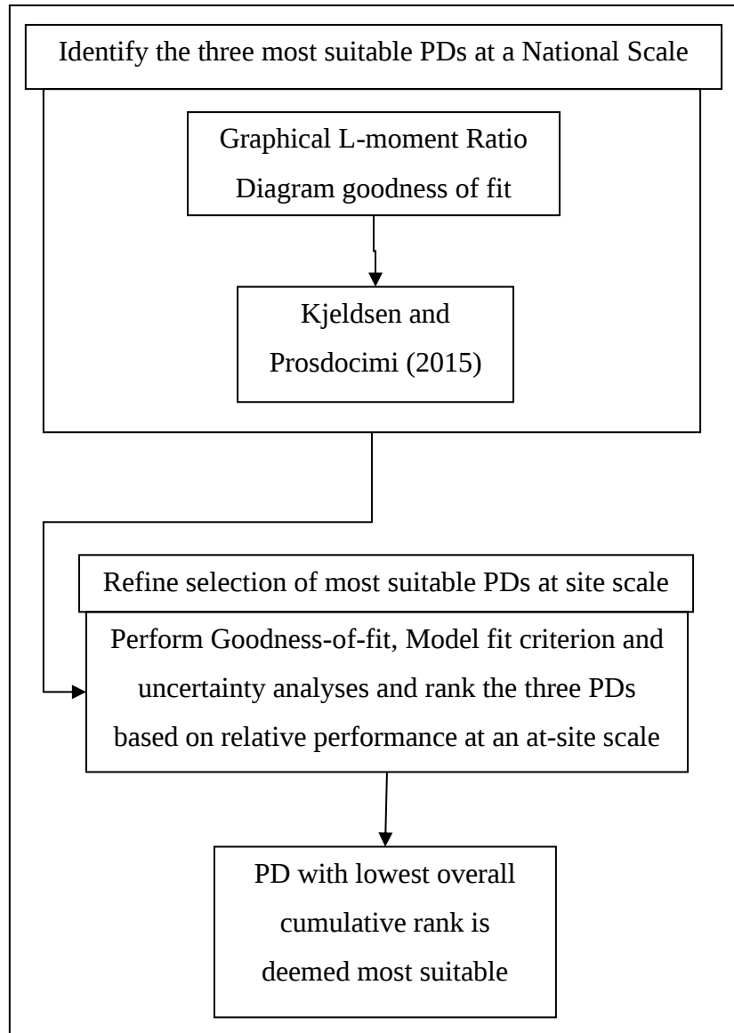
Figure 3.3 Methodology flow diagram for the selection of a suitable parent distribution
