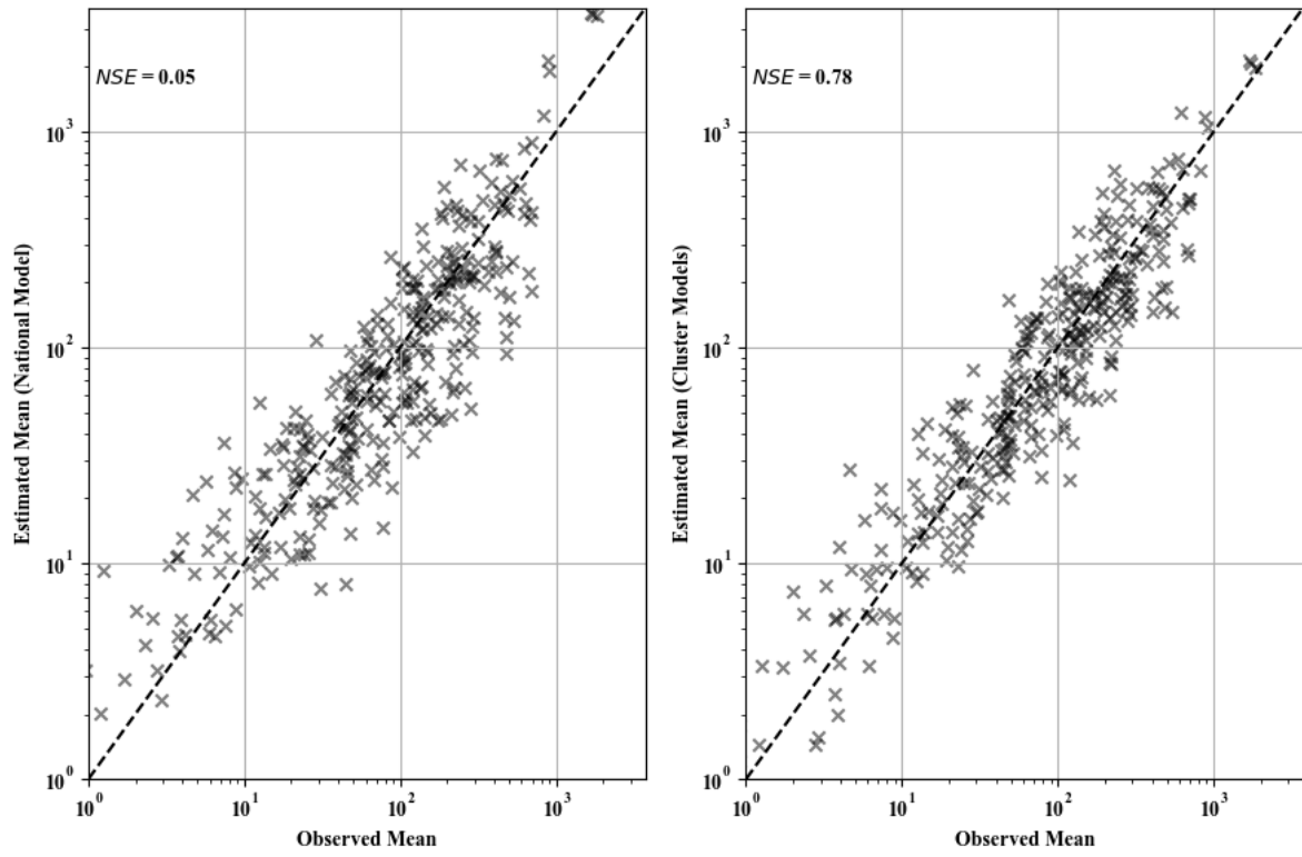
Figure 8.3 Observed versus estimated MAF for the national- (left) and cluster based (right) models
