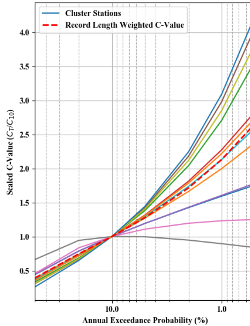
Dimensionless Peak Flow and Scaled C-value - Cluster 5
