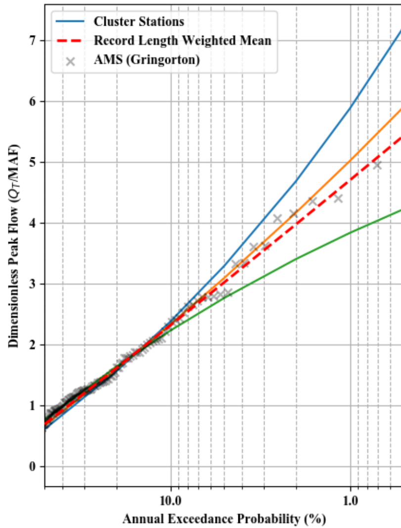
Dimensionless Peak Flow and Scaled C-value - Cluster 19
