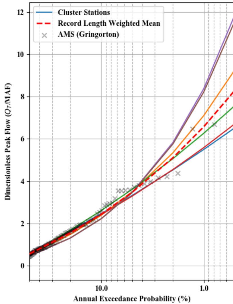
Dimensionless Peak Flow and Scaled C-value - Cluster 12
