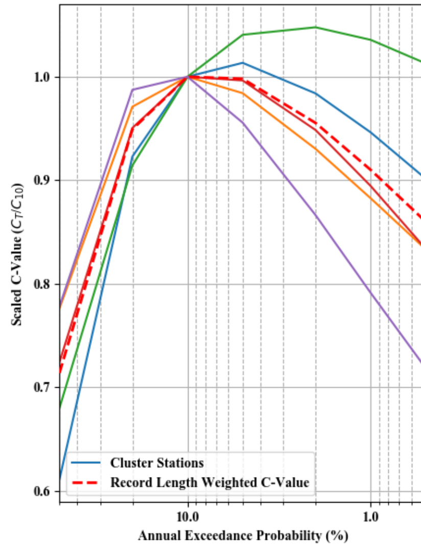
Dimensionless Peak Flow and Scaled C-value - Cluster 23
