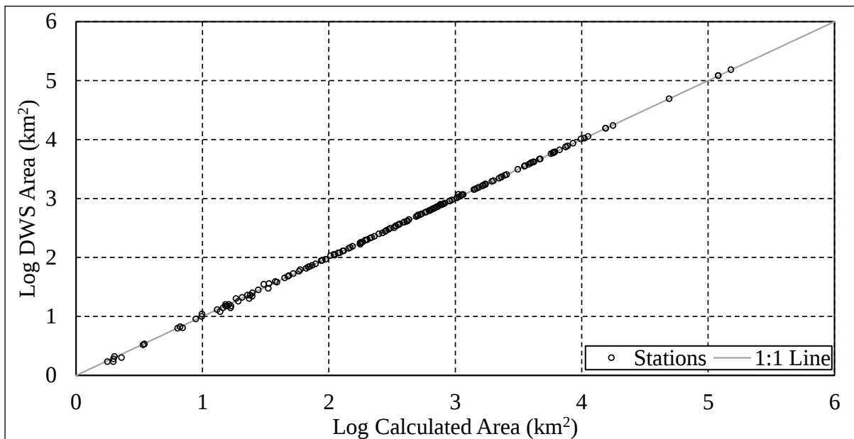
Figure 4.1 Catchment area comparison
