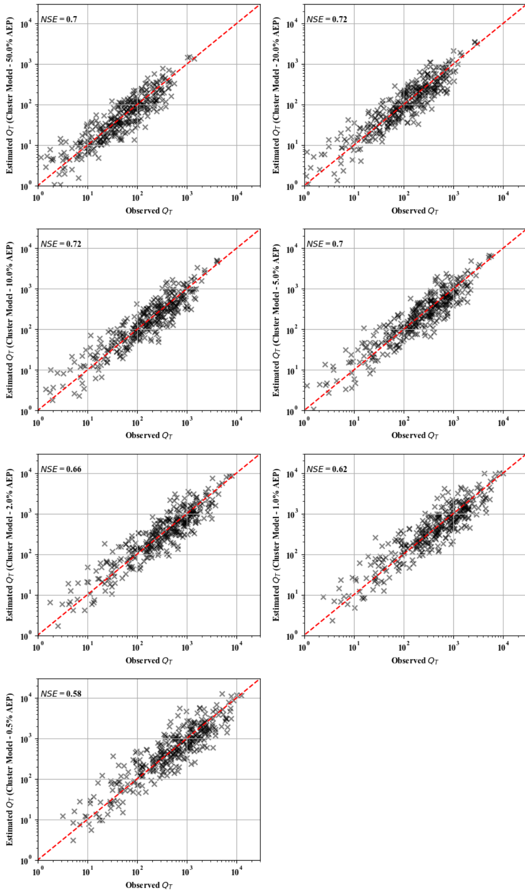
Figure 8.7 Estimated vs observed Q_T using the RIF Cluster based approach for the 50, 20, 10, 5, 2, 1 and 0.5% annual exceedance probabilities
