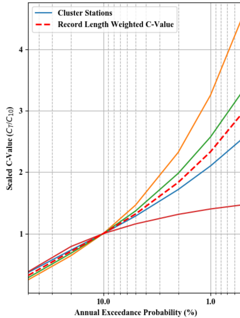
Dimensionless Peak Flow and Scaled C-value - Cluster 18
