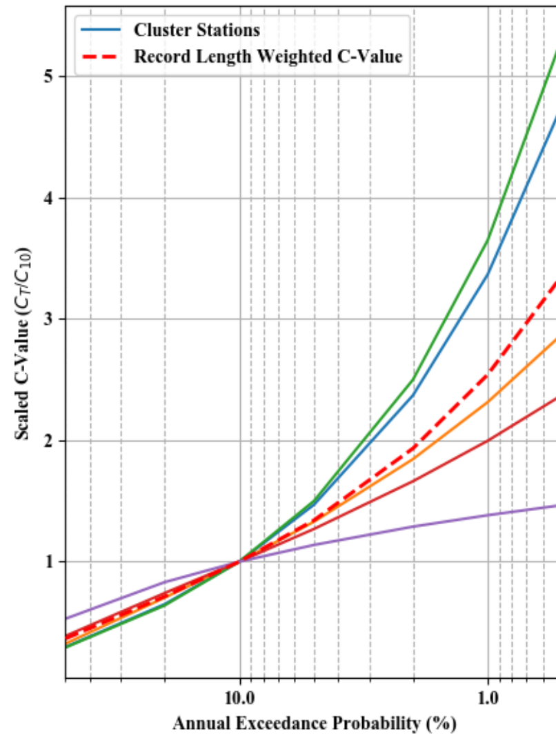
Dimensionless Peak Flow and Scaled C-value - Cluster 3
