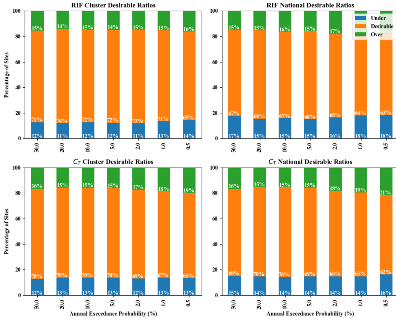
Figure 8.8 Percentage of Q_T estimates within the desirable ratio defined by Rahman et al. (2012) using the RIF (top) and C_T (bottom) approaches for both Cluster based and National based scaling factor estimation methods
