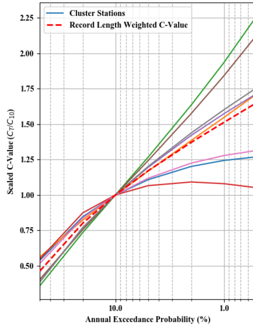
Dimensionless Peak Flow and Scaled C-value - Cluster 10
